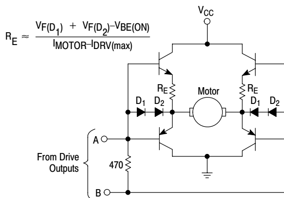
Figure 28. Bridge Amplifier
