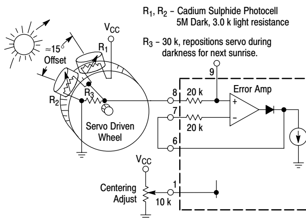
Figure 19. Solar Tracking Servo System
