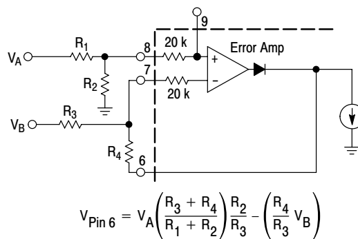
Figure 26. Differential Input Amplifier
