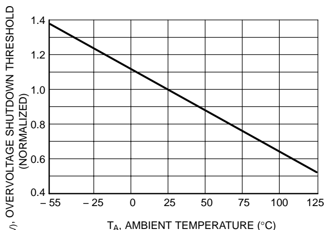
Figure 14. Normalized Overvoltage Shutdown Hysteresis versus Temperature
