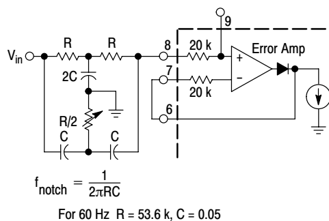
Figure 25. Notch Filter
