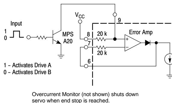
Figure 22. Digital Two Position Servo System
