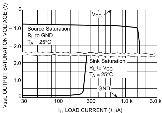
Figure 2. Error Amp Output Saturation versus Load Current
