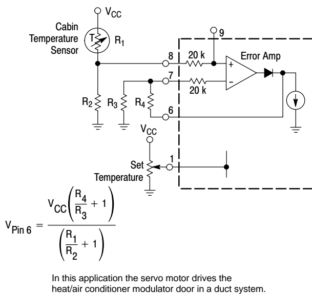
Figure 27. Temperature Sensing Servo System
