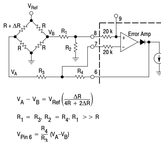
Figure 28. Bridge Amplifier
