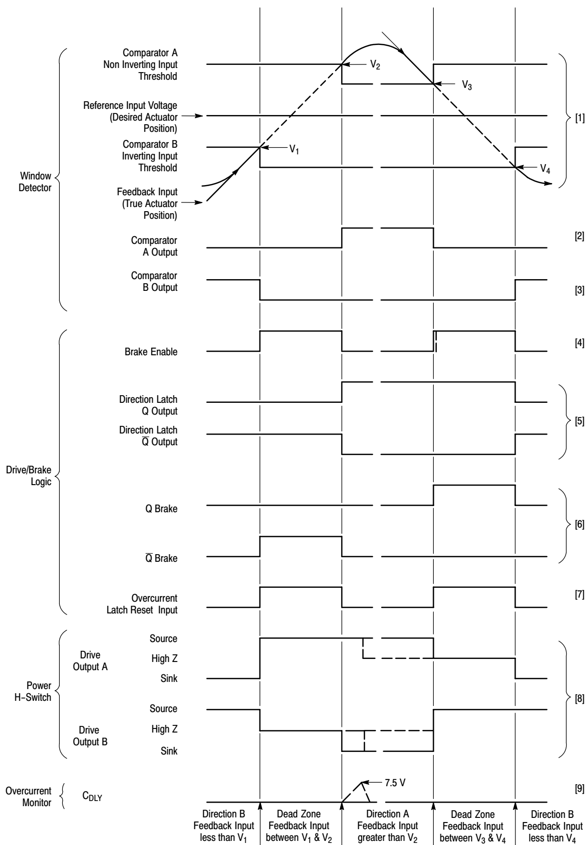
Figure 18. Timing Diagram
