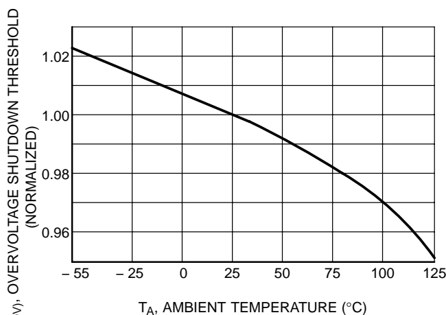
Figure 13. Normalized Overvoltage Shutdown Threshold versus Temperature
