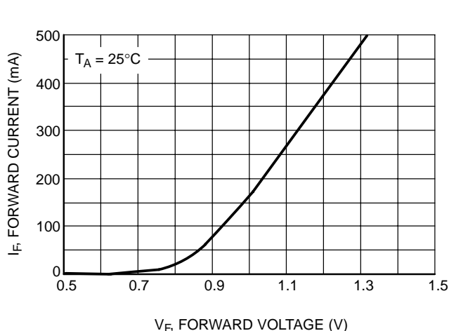
Figure 7. Brake Diode Forward Current versus Forward Voltage
