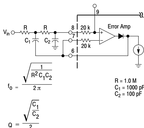
Figure 24. Second Order Low-Pass Active Filter Servo System
