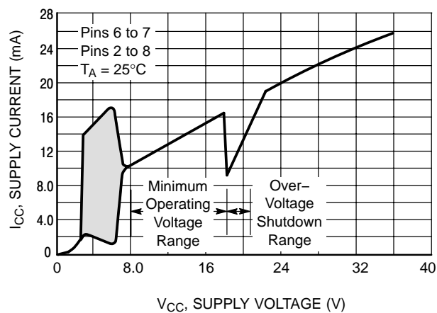
Figure 12. Supply Current versus Supply Voltage
