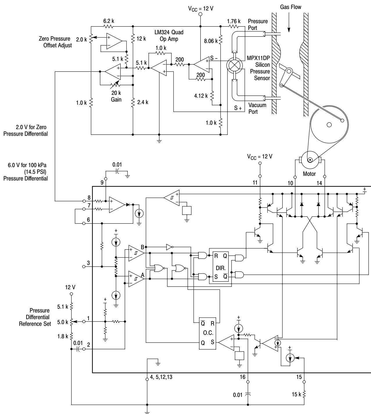
Figure 31. Adjustable Pressure Differential Regulator
