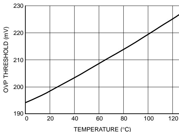
Figure 5. OVP Threshold above VID versus Temperature
