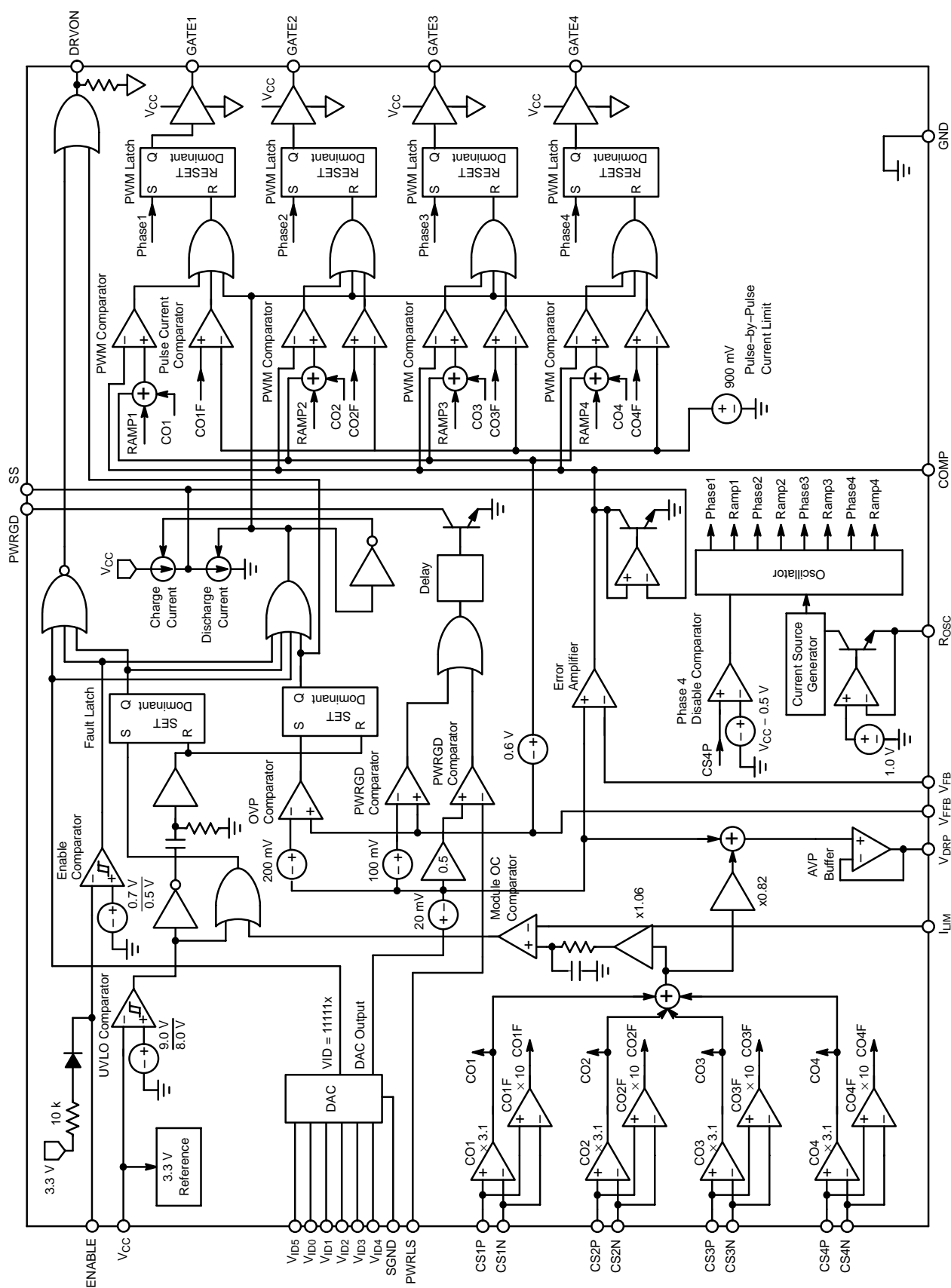
Figure 2. Block Diagram
