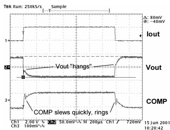
Figure 34. The Value of C_{AMP} Is Too Low and the Loop Gain/Bandwidth Too High. COMP Moves Too Quickly, Which Is Evident from the Small Spike in Its Voltage When the Load Is Applied or Removed. The Output Voltage Transitions More Slowly Because of the COMP Spike.
