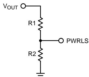
Figure 23. Adjusting the PWRGD Threshold
