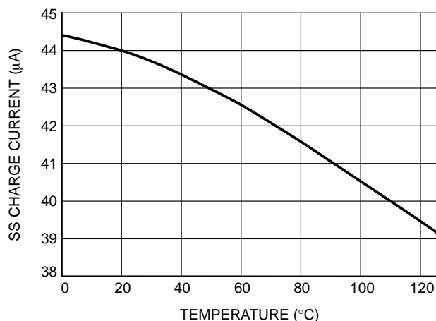
Figure 11. Soft-Start Charge Current versus Temperature
