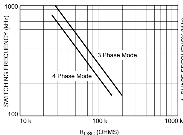
Figure 7. Oscillator Frequency versus Total R_{OSC} Value
