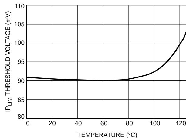
Figure 14. Pulse-by-Pulse Current Limit Threshold versus Temperature
