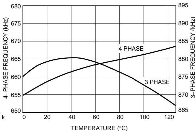
Figure 8. Switching Frequency versus Temperature ( R_{OSC} = 32.4 \text{ k}\Omega )
