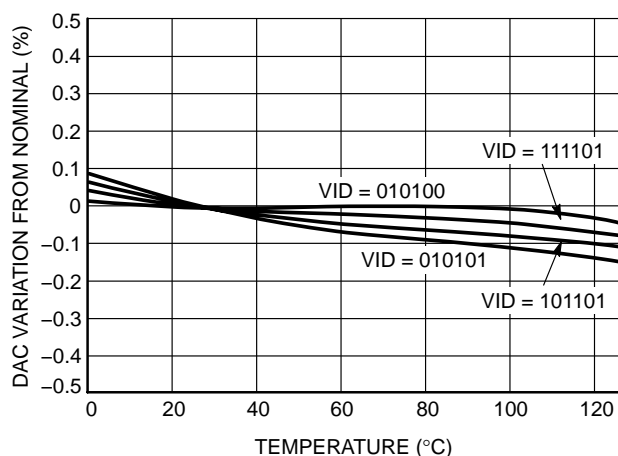
Figure 3. DAC Variation versus Temperature
