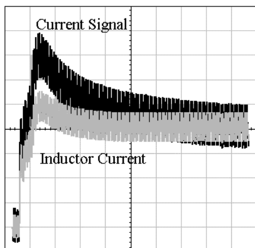
Figure 20. Inductive Sensing Waveform During a Load Step with Fast RC Time Constant (50 \mu s/div)
