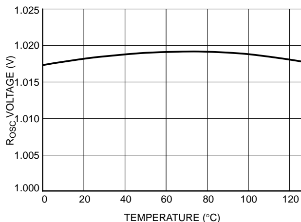
Figure 9. V ROSC versus Temperature
