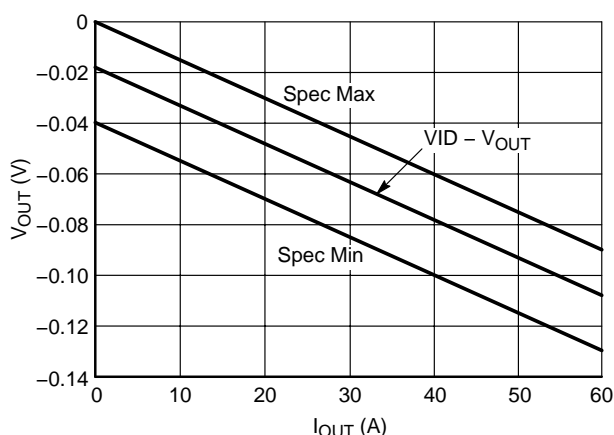
Figure 29. The DC Effects of AVP vs. Load
