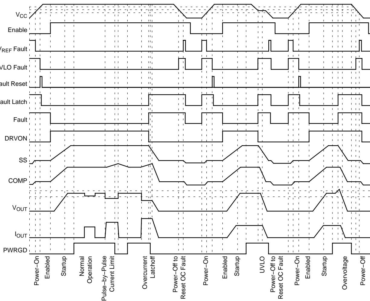
Figure 16. Operating Waveforms
