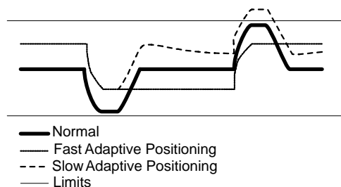
Figure 21. Adaptive Voltage Positioning
