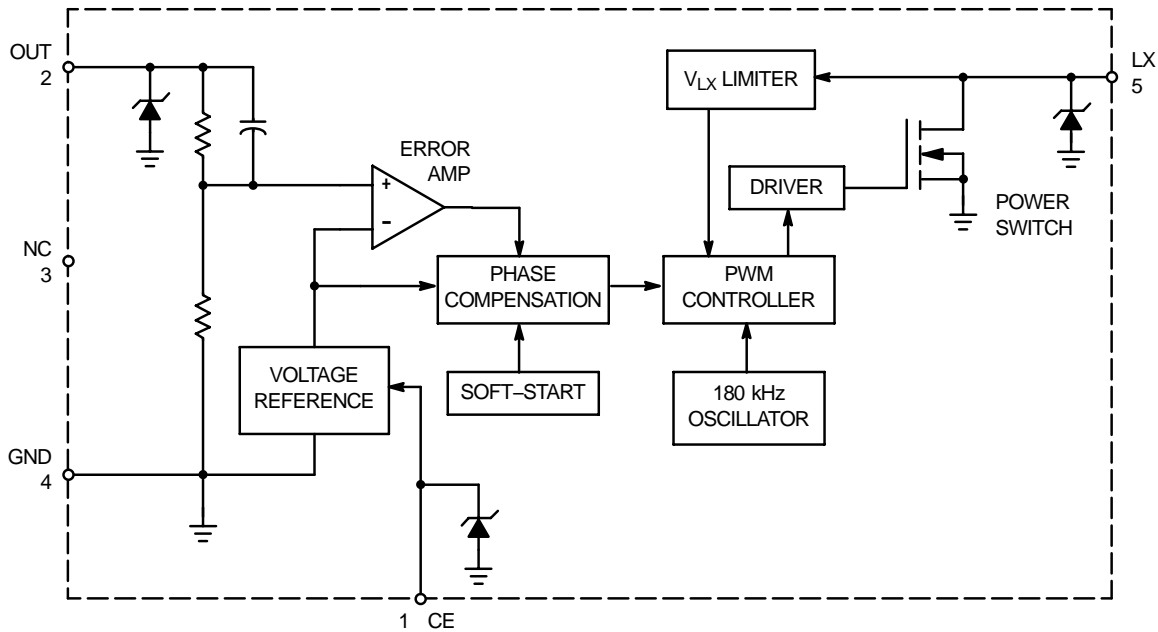
Figure 40. Representative Block Diagram
