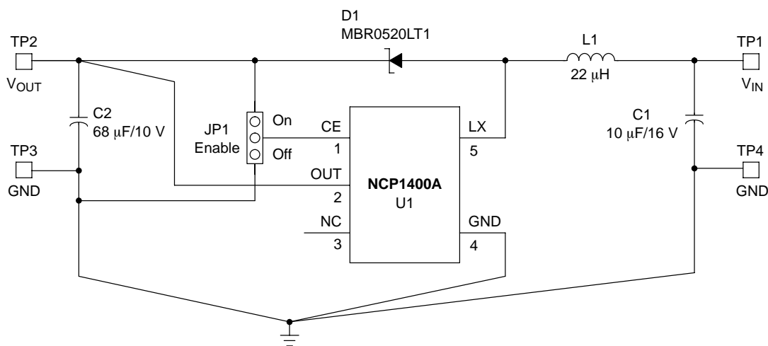
Figure 44. NCP1400A Evaluation Board Schematic Diagram
