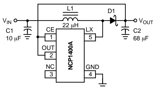
Figure 41. Typical Step-Up Converter Application
