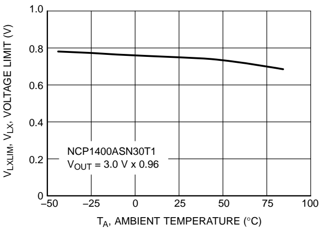
Figure 12. NCP1400ASN30T1 V_{LX} Voltage Limit vs. Temperature
