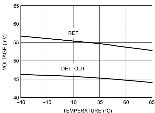
Figure 4. Detector and Reference Output Variation Overtemperature ( V_{CC} = 2.7 V, No RF Applied)
