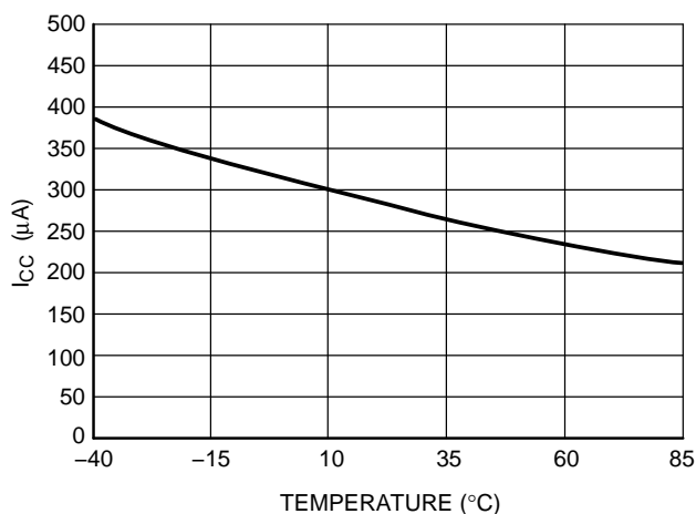
Figure 8. I_{CC} Variation Overtemperature ( V_{CC} = 5.5 V, No RF Applied)
