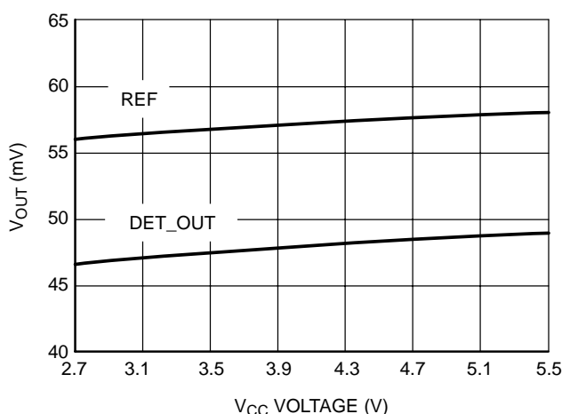
Figure 6. Detector and Reference Output Variation Over V_{CC} Bias ( T_A = 25^\circ\text{C} , No RF Applied)
