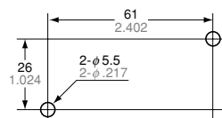
Mounting dimension
