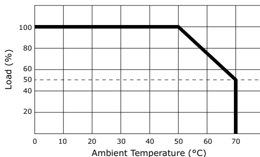
output power vs. ambient temperature
