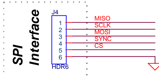
Figure 6 SPI interface connector
