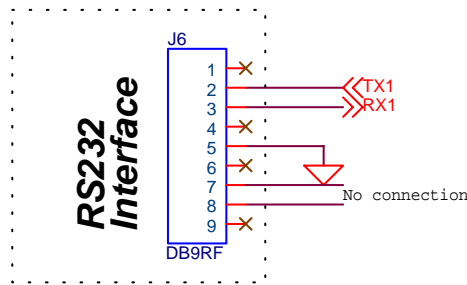
Figure 5. RS232C connector
