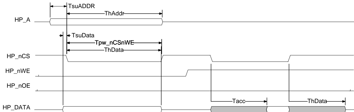
Figure 9. Register Write/Read Timing (Motorola)
