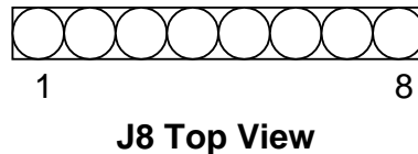
Figure 5. J8 Connector connection
