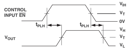
Figure 2. Propagation Delay
