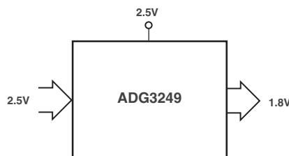
Figure 7. 2.5 V to 1.8 V Voltage Translation, \overline{SEL} = 2.5 V_{CC}
