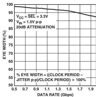
TPC 19. Eye Width vs. Data Rate; PRBS 31
