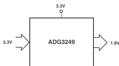
Figure 9. 3.3 V to 1.8 V Voltage Translation, \overline{SEL} = 0 V
