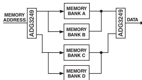
Figure 12. ADG3249 Used to Reduce Both Access Time and Noise
