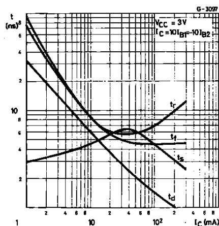
Switching Characteristics.
