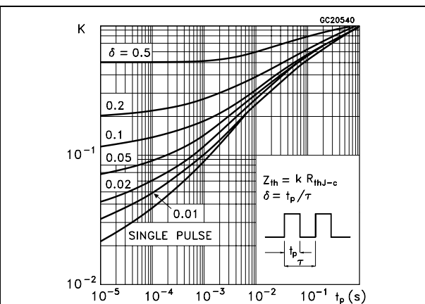
Figure 4. Thermal impedance for TO-220/D 2 PAK
