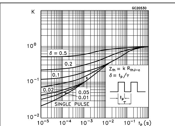
Figure 8. Thermal impedance for TO-247
