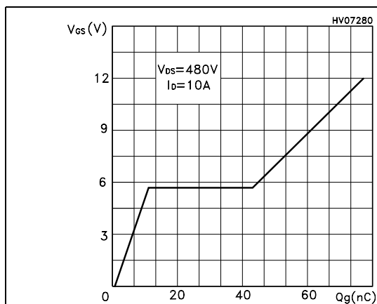
Figure 13. Gate charge vs gate-source voltage
