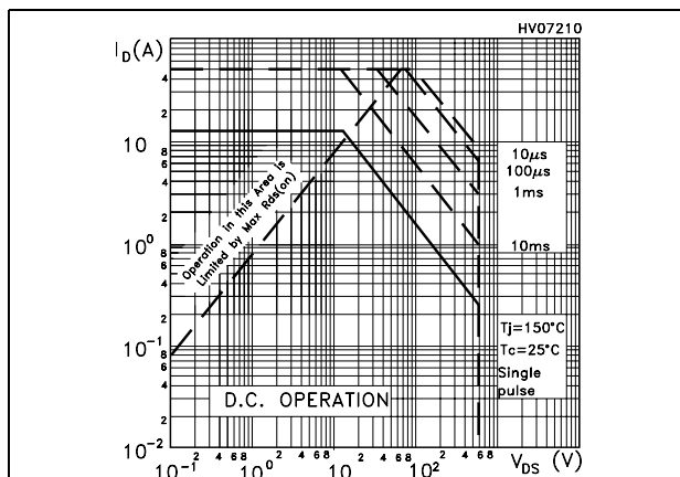
Figure 3. Safe operating area for TO-220/D 2 PAK
