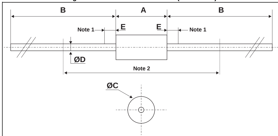
Figure 18. DO-201AD dimensions (definitions)
