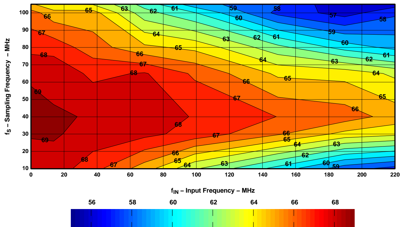
Figure 14. SNR– dBFS
