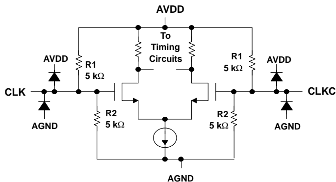
Figure 28. Clock Inputs
