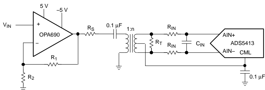
Figure 31. Converting a Single-Ended Input Signal Into a Differential Signal Using an RF Transformer
