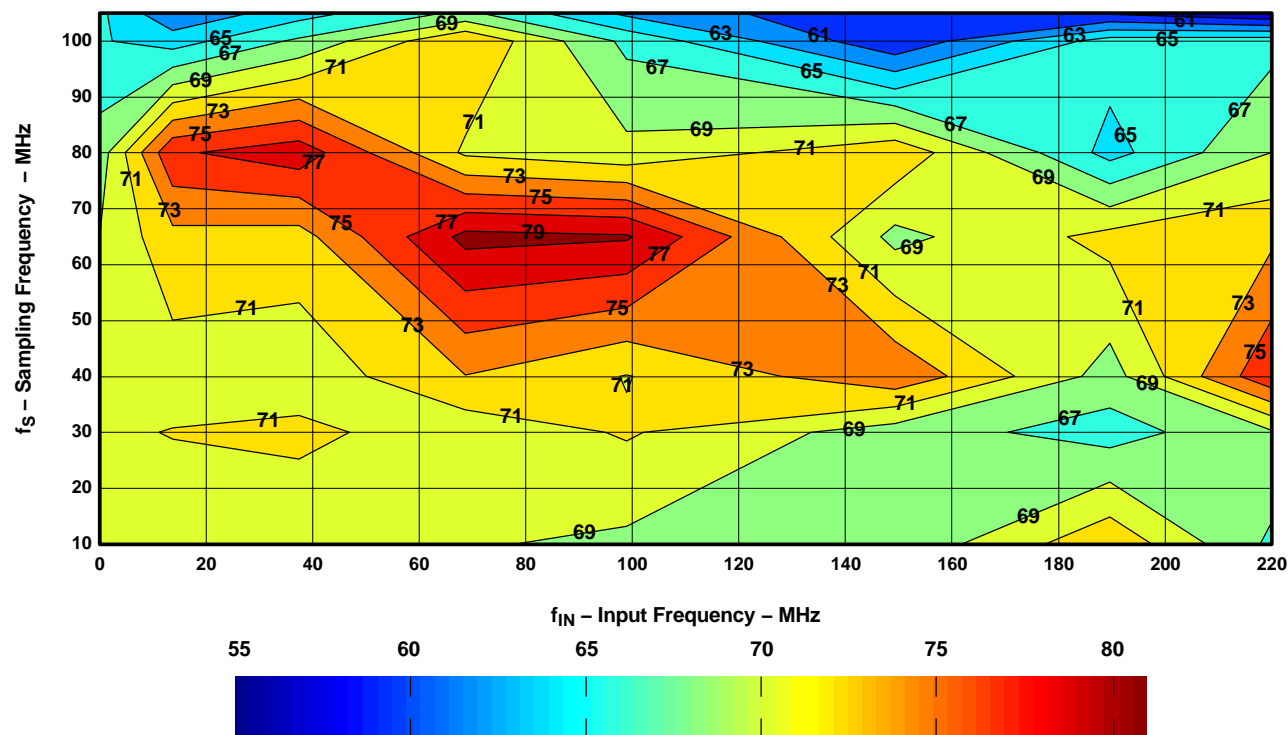
Figure 15. SFDR – dBc
