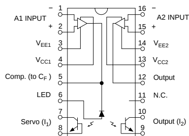
LIA100/LIA101 Pinout
