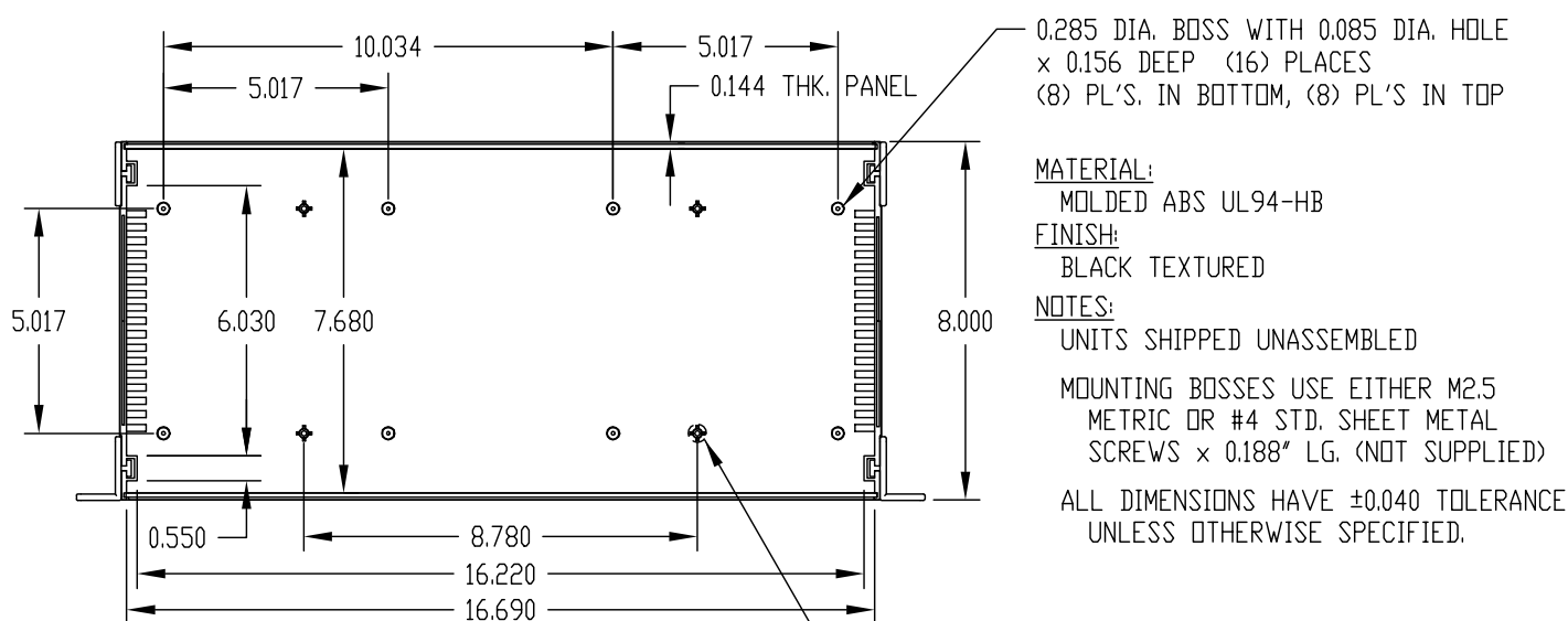
TOP VIEW (LESS TOP)
