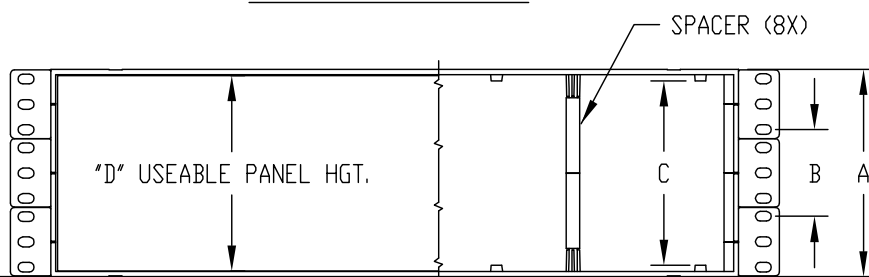
FRONT VIEW 2U HEIGHT
