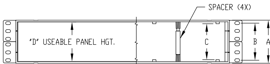
FRONT VIEW 2U HEIGHT
