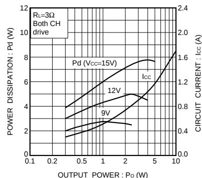
Fig.30 Power dissipation and current dissipation vs.power supply voltage ( R_L=3\Omega )
