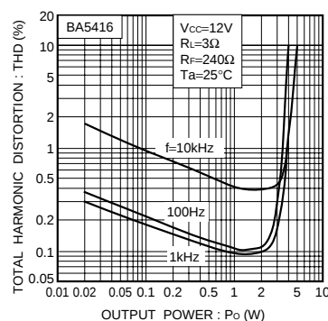
Fig.15 Total harmonic distortion vs. output power (BA5416)
