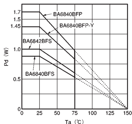
Fig.1 Power dissipation curves
