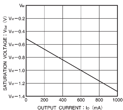
Fig.4 High-level output saturation voltage vs. output current
