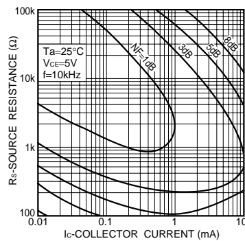
Fig.22 Noise characteristics (IV)
