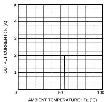
Fig.6 Derating curve
