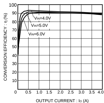
Fig.16 Conversion efficiency
