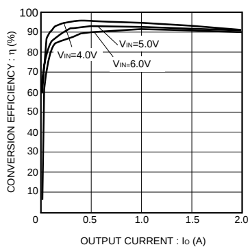
Fig.10 Conversion efficiency
