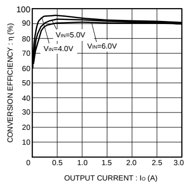
Fig.13 Conversion efficiency
