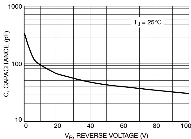
Figure 4. Typical Capacitance
