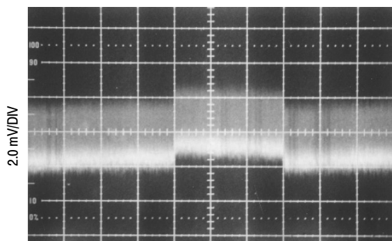
Figure 10. Reference Line Regulation 10 V to 24 V (2.0 ms/DIV)
