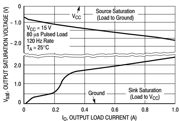
Figure 15. Output Saturation Voltage versus Load Current
