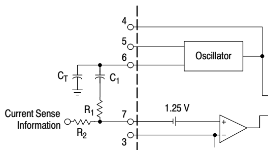
Figure 24. Resistive Current Sensing
