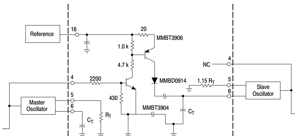
Figure 30. Synchronization Over Long Distances
