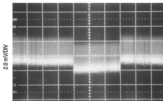
Figure 11. Reference Load Regulation 1.0 mA to 10 mA (2.0 ms/DIV)
