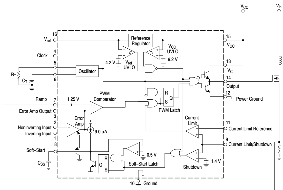
Figure 19. Representative Block Diagram
