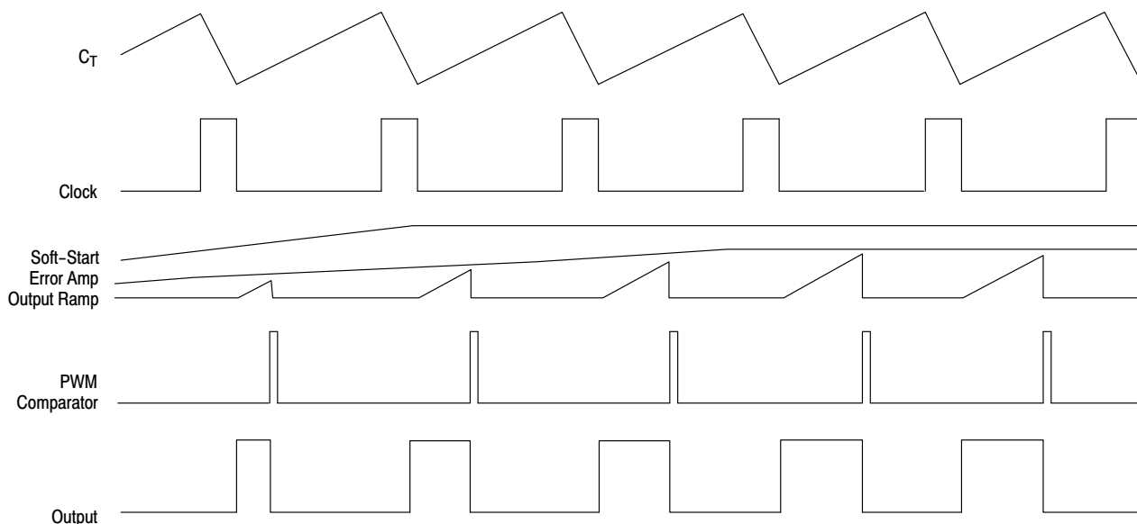
Figure 20. Current Limit Operating Waveforms
