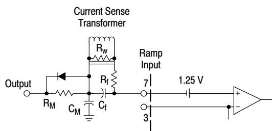
Figure 26A. Slope Compensation (Noise Sensitive)
