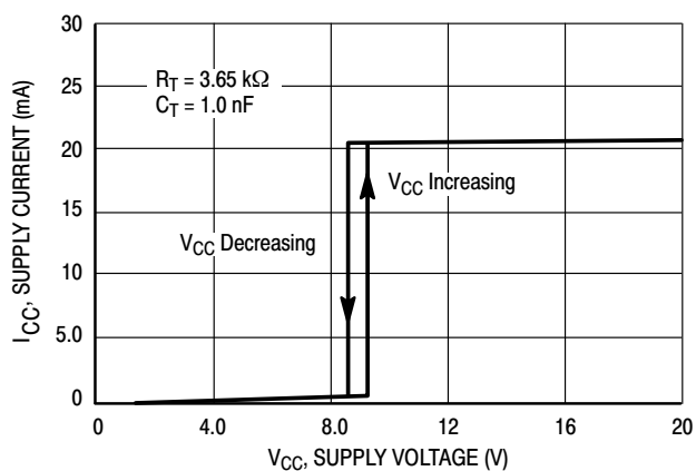
Figure 18. Supply Voltage versus Supply Current
