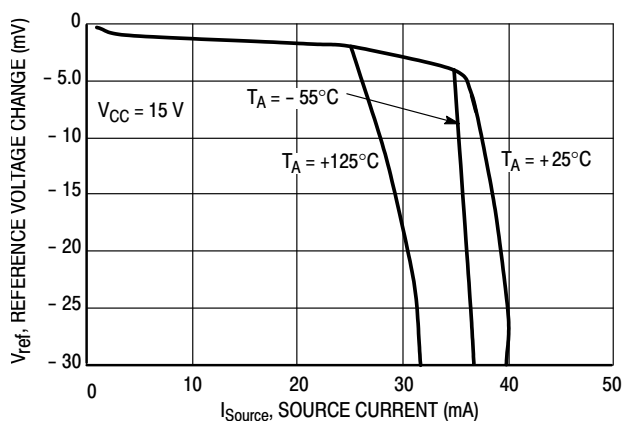
Figure 8. Reference Voltage Change versus Source Current
