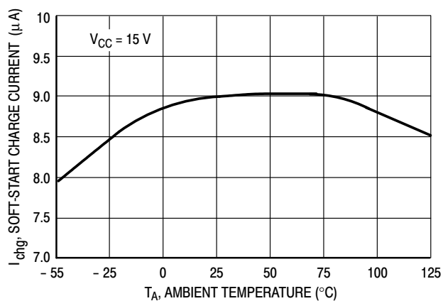
Figure 14. Soft-Start Charge Current versus Temperature
