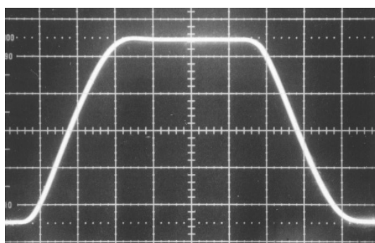
Figure 17. Drive Output Rise and Fall Time
