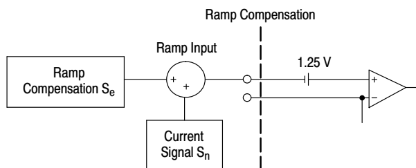
Figure 21. Ramp Compensation
