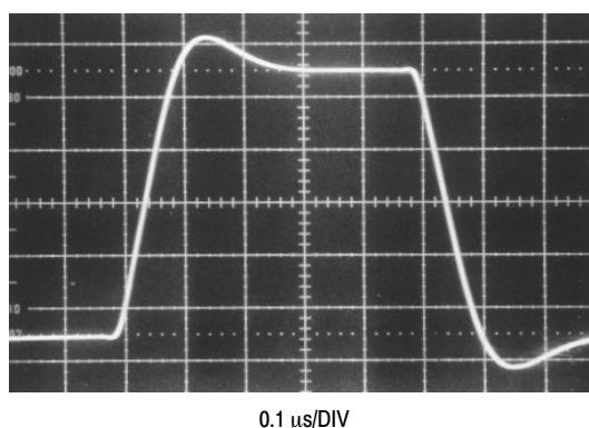
Figure 7. Error Amp Large Signal Transient Response
