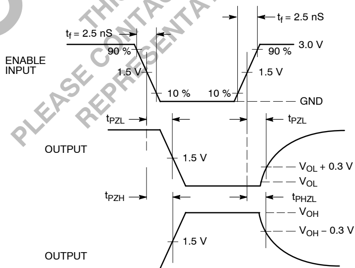
Figure 5. Enable/Disable Delays
