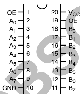
Figure 1. 20-Lead Pinout
