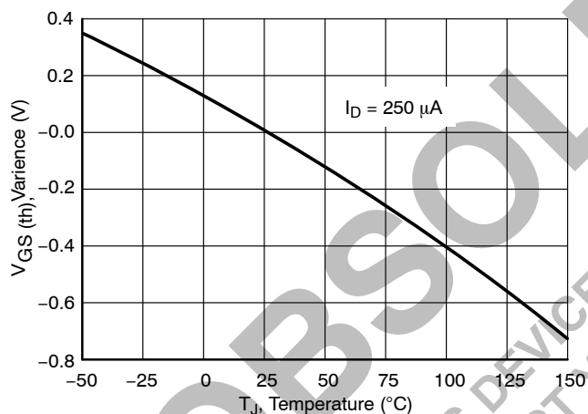
Figure 9. Threshold Voltage
