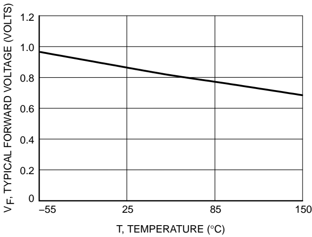
Figure 7. Forward Voltage
