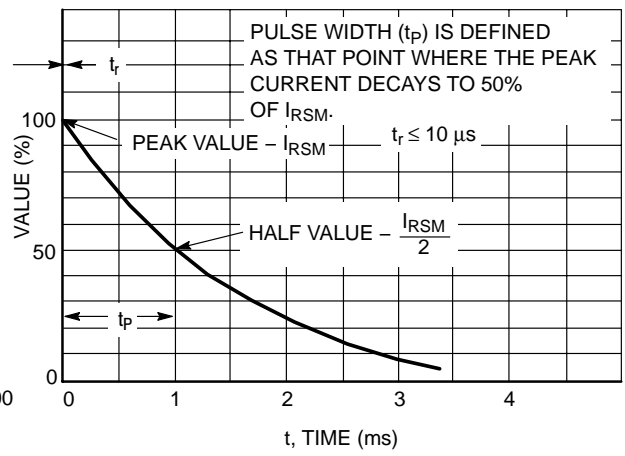
Figure 2. 10 X 1000 µs Pulse Waveform
