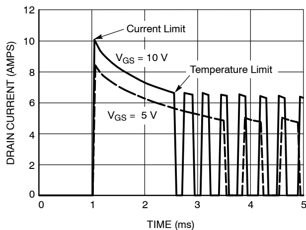
Figure 9. Short-circuit Response
