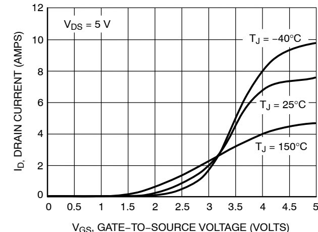
Figure 4. Transfer Characteristics
