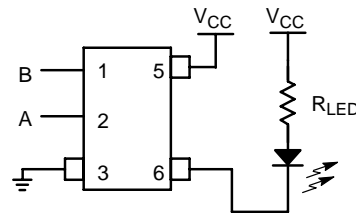
Figure 8. LED Driver
