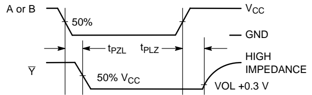
Figure 5. Switching Waveforms
