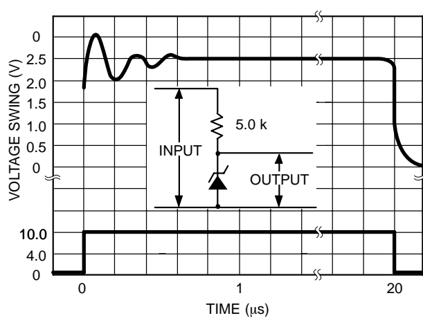
Figure 8. Response Time
