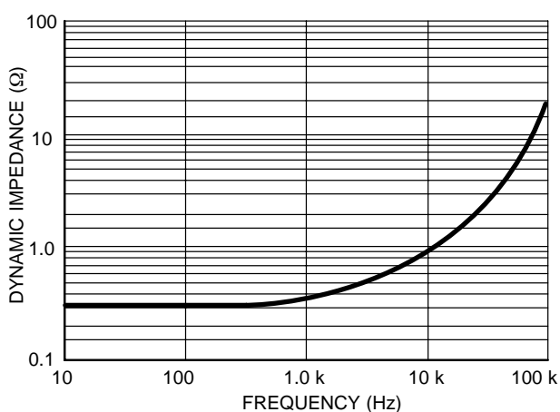
Figure 6. Dynamic Impedance vs. Frequency
