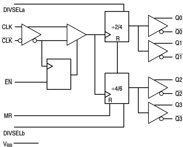
Figure 2. Logic Diagram
