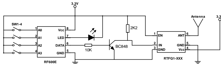
Transmitter Circuit
