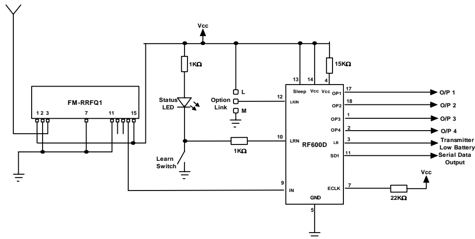
Receiver Circuit
