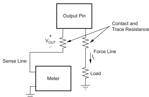
Figure 23. Accurate Load Regulation of REF31xx
