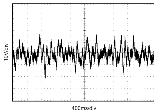
Figure 21. 0.1-Hz to 10-Hz Noise
