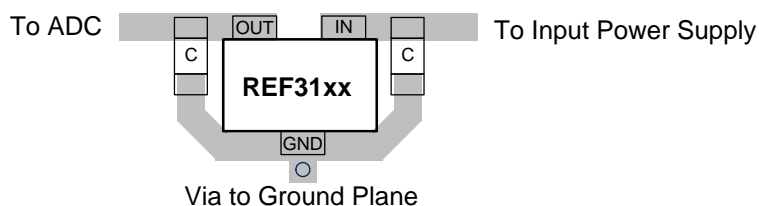
Figure 33. Layout Example
