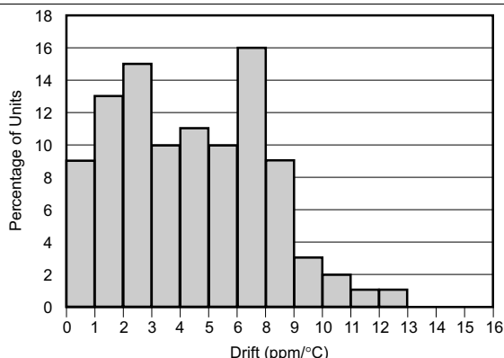
Figure 1. Temperature Drift (0°C to 70°C)
