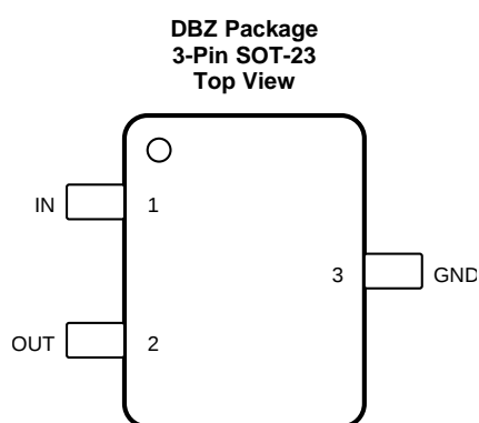
Pin Functions
