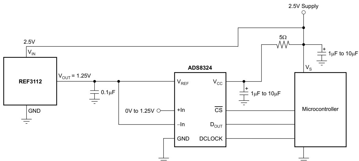
Figure 26. Basic Data Acquisition System 2
