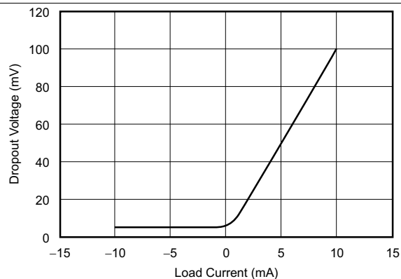
Figure 4. Dropout Voltage vs Load Current
