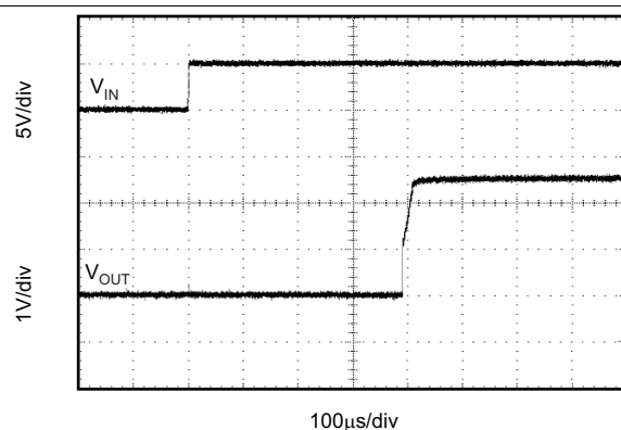
Figure 10. Step Response, C_L = 0 , 5-V Start-Up
