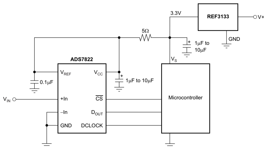
Figure 25. Basic Data Acquisition System 1
