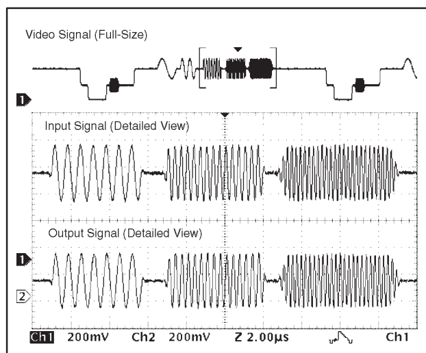
Figure 3. Multiburst (CCIR 18) Test Pattern (PAL)
