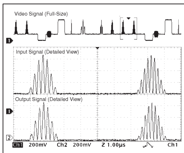
Figure 4. Multipulse Test Pattern (PAL)
