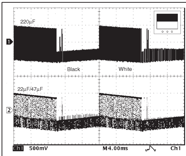
Figure 10. Standard Video Circuit with 220 \mu F Capacitor (top trace) vs OPA360 with 22 \mu F and 47 \mu F Capacitors
