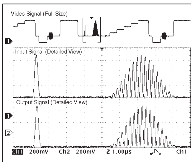
Figure 5. CCIR 17 Test Pattern (PAL)
