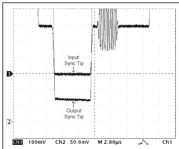
Figure 6. Internal Level Shifter, Shifts Input Signal by Approximately 60mV to Prevent Sync Clipping
