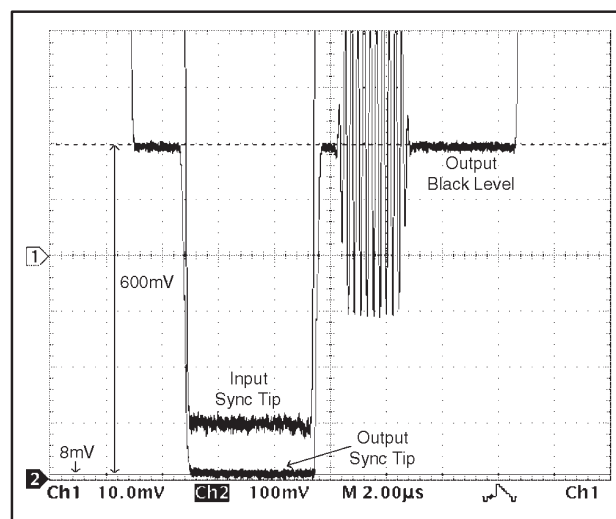
Figure 8. Input Sync Tip at -30mV (Output Shows No Sign of Clipping)
