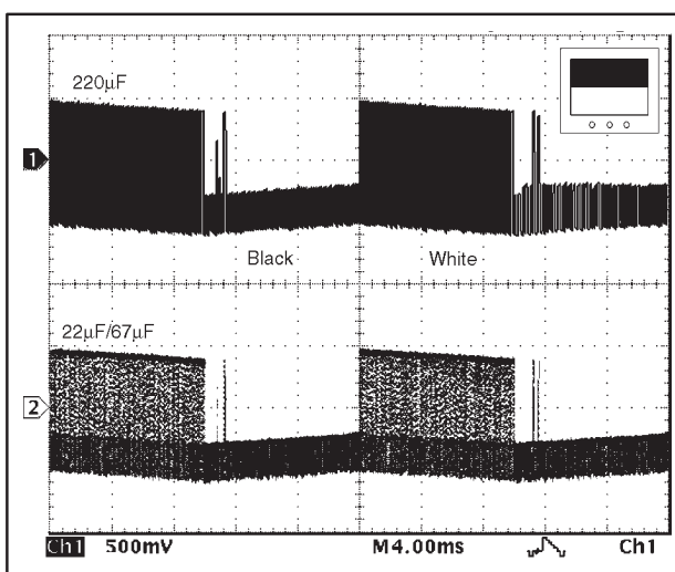
Figure 11. 220 \mu F Standard Video Circuit (top trace) vs OPA360 with 22 \mu F and 67 \mu F Capacitors
