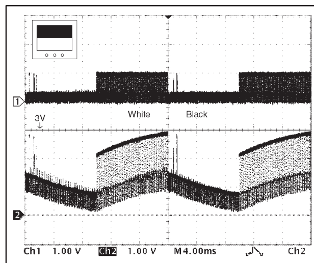
Figure 7. Output Swing with 33μF on 3V Supply
