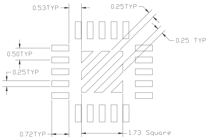
Stencil Aperture All Dimensions in mm
