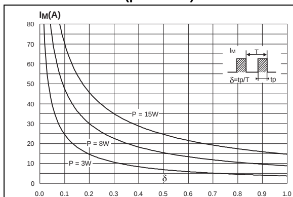
Figure 1. Peak current versus duty cycle (per diode)
