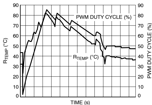
Figure 79. Fan Reaction to Temperature Variation in Enhanced Acoustics Mode
