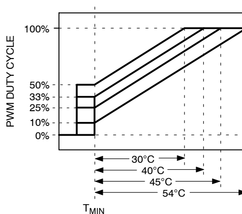
Figure 62. Increasing \text{PWM}_{\text{MIN}} Changes Effective T_{\text{RANGE}}
