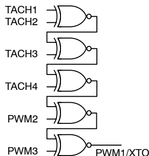
Figure 46. XNOR Tree Test
