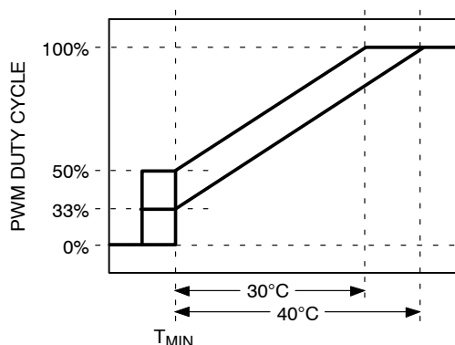
Figure 61. Adjusting \text{PWM}_{\text{MIN}} Affects T_{\text{RANGE}}
