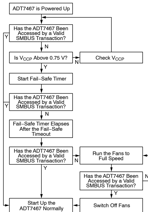
Figure 47. Power-On Flowchart
