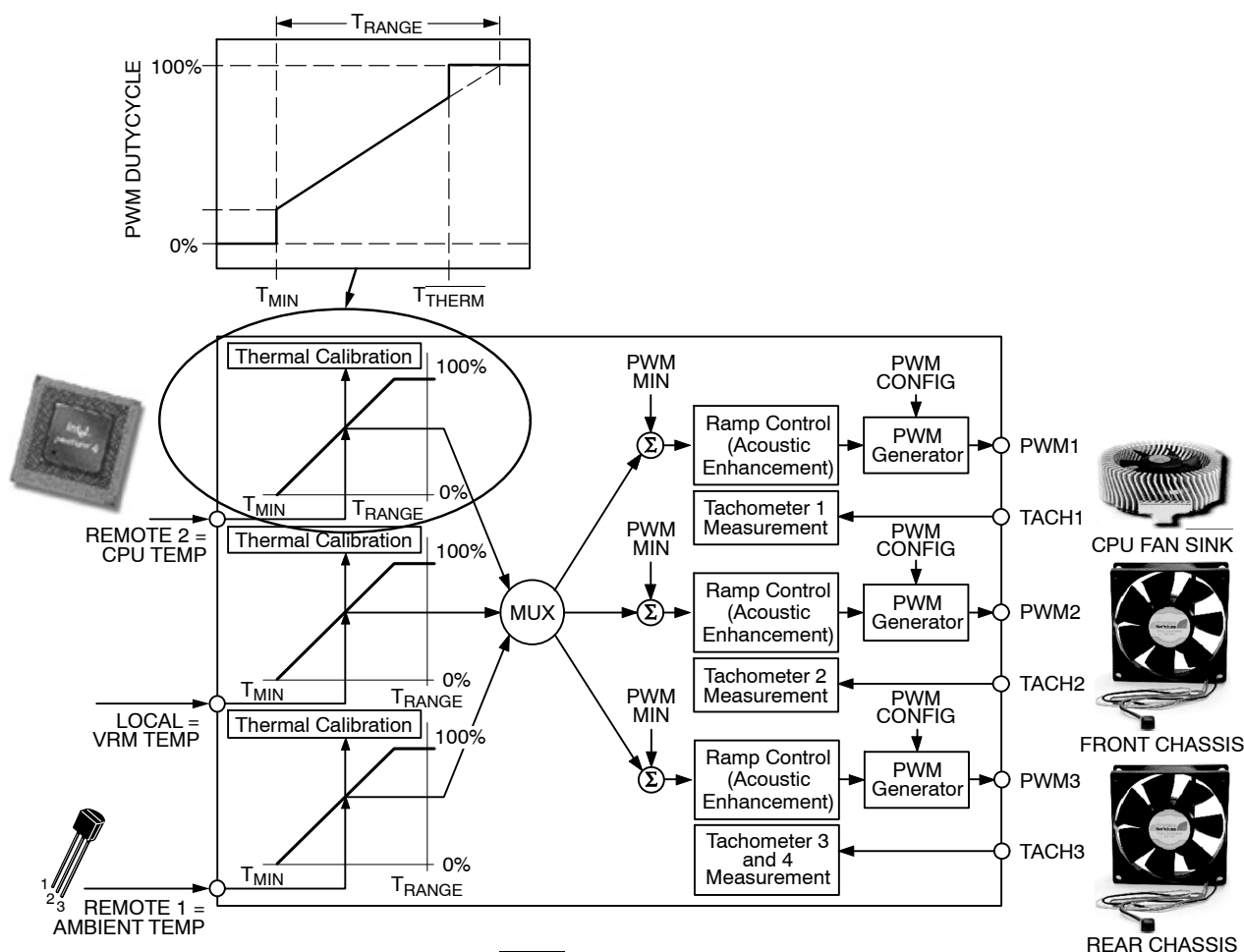
Figure 66. How T_{THERM} Relates to Automatic Fan Control
