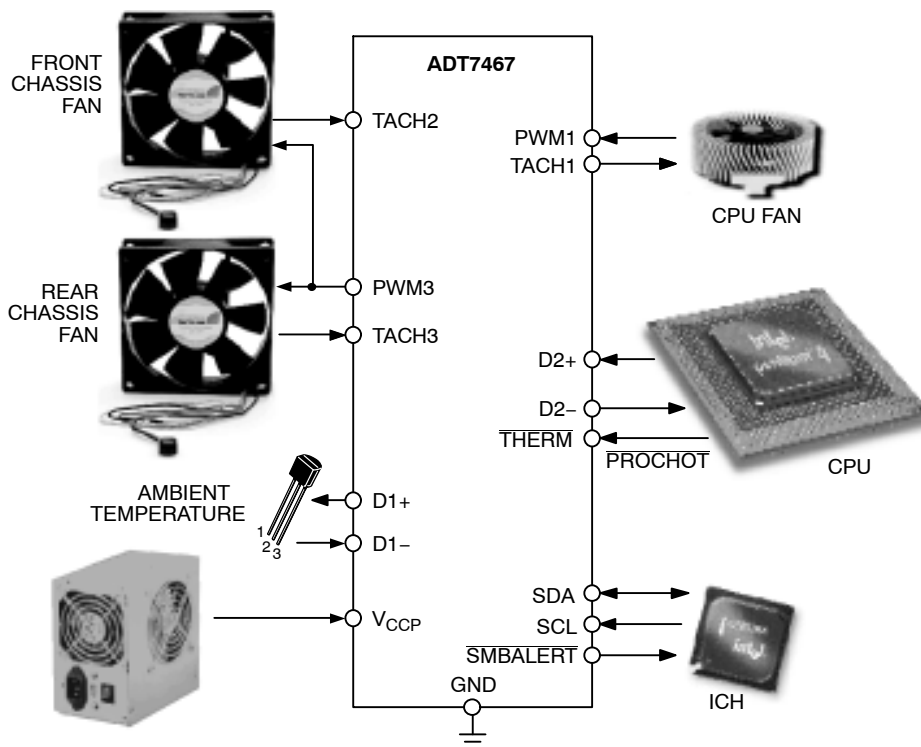
Figure 53. Recommended Implementation
