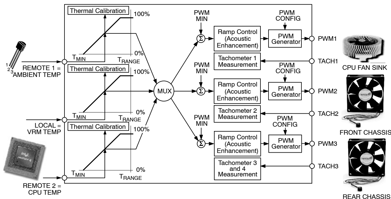
Figure 52. Hardware Configuration Example
