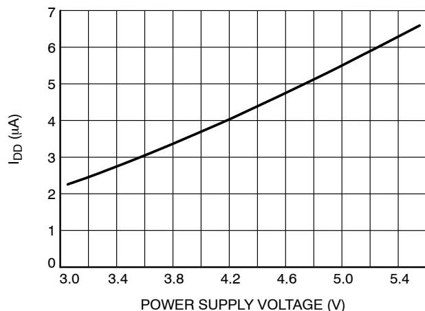
Figure 9. Shutdown I_{DD} vs. Power Supply
