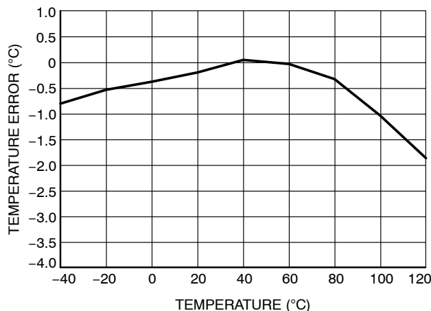
Figure 10. Internal Temperature Error vs. Temperature
