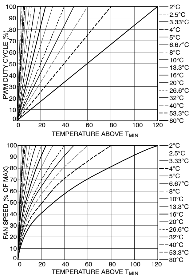
Figure 63. T_{RANGE} vs. Fan Speed Profile
