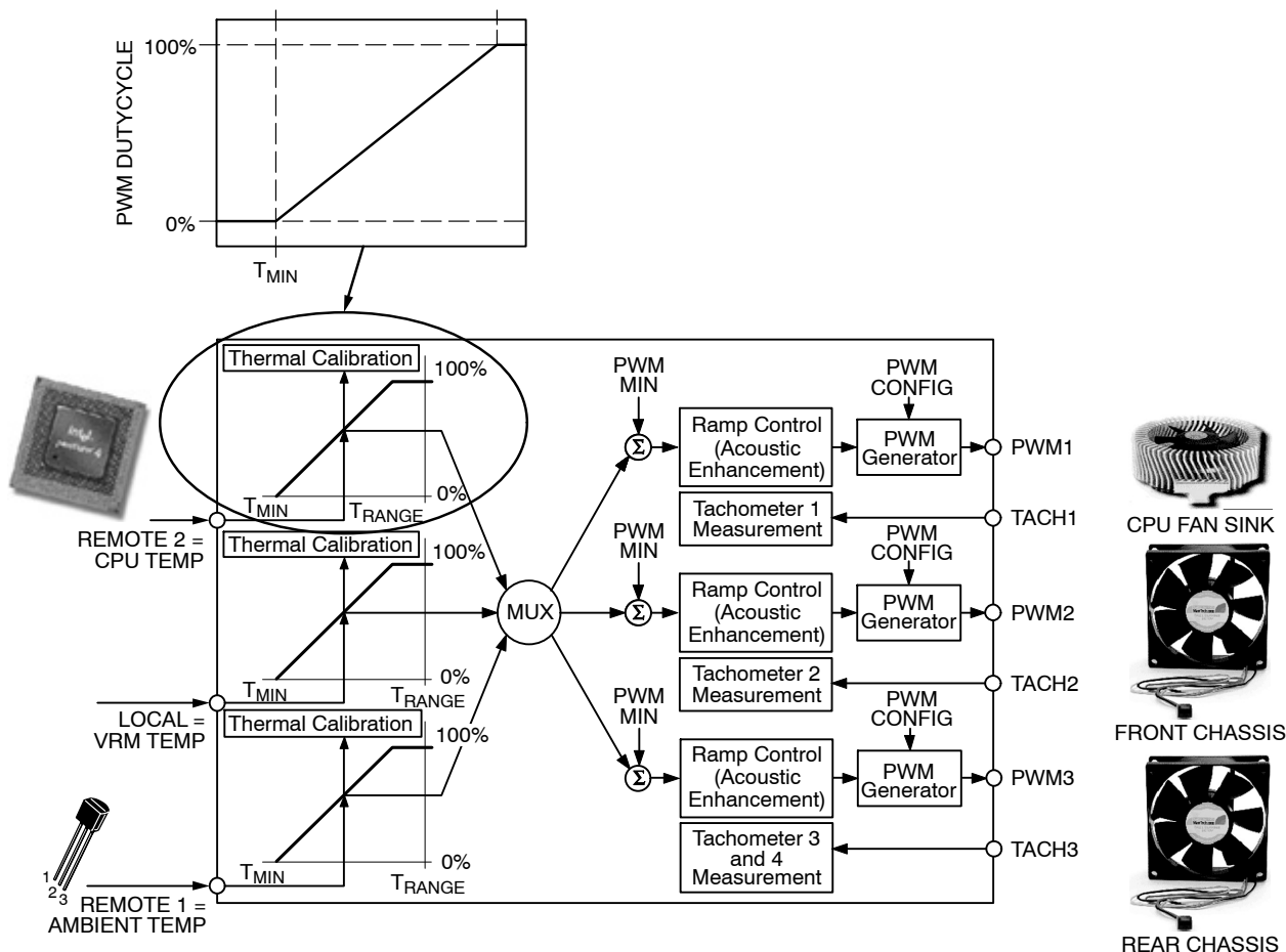
Figure 56. Understanding the T_{MIN} Parameter
