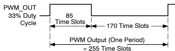
Figure 81. 33% PWM Duty Cycle, Represented in Time Slots
