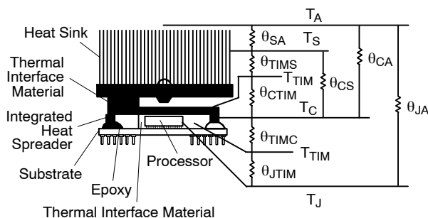
Figure 50. Thermal Model
