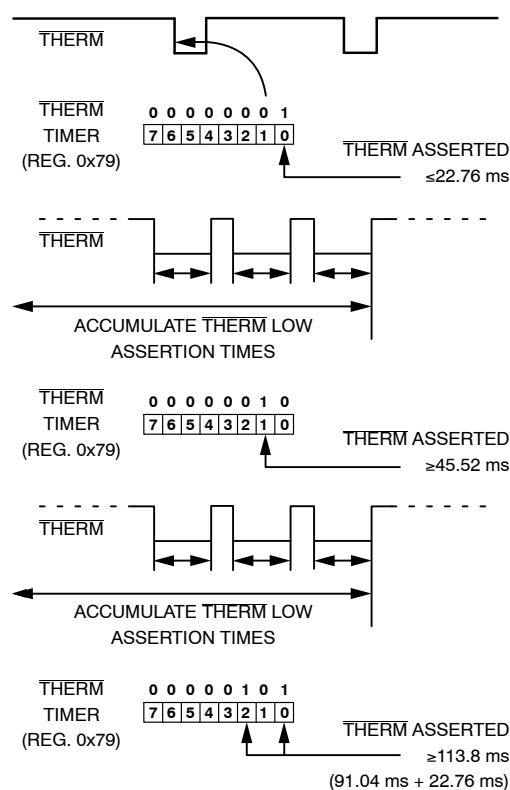
Figure 30. Understanding the THERM Timer
