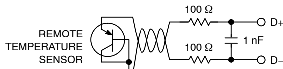
Figure 23. Filter Between Remote Sensor and ADT7467
