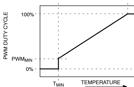
Figure 57. PWM_{MIN} Determines Minimum PWM Duty Cycle
