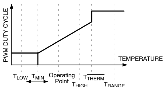
Figure 51. Dynamic T_{MIN} Control Loop
