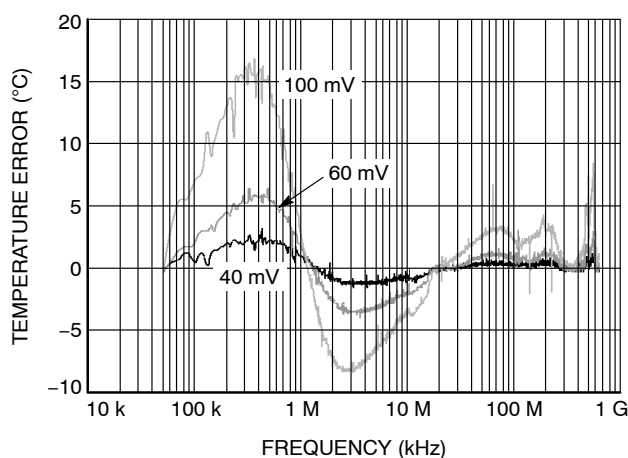
Figure 4. Remote Temperature Error vs. Common-Mode Noise Frequency
