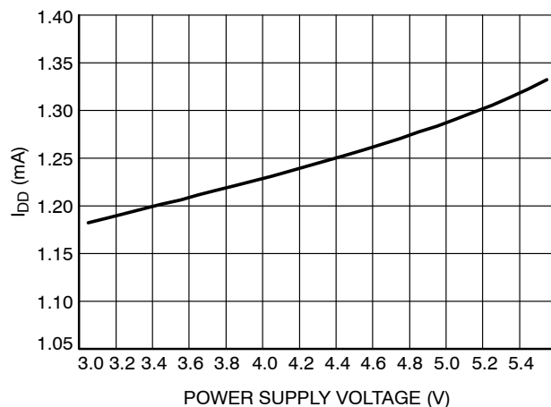
Figure 8. Normal I_{DD} vs. Power Supply
