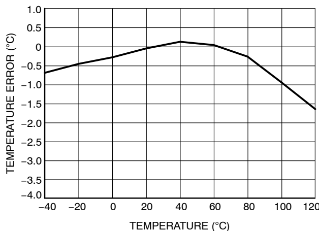
Figure 12. Remote Temperature Error vs. Temperature
