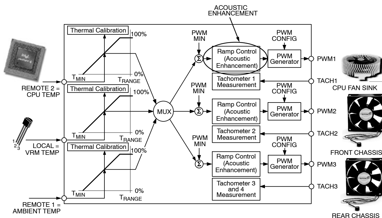
Figure 80. Acoustic Enhancement Smoothes Fan Speed Variations in Automatic Fan Speed Control
