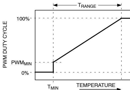
Figure 60. T_{\text{RANGE}} Parameter Affects Cooling Slope
