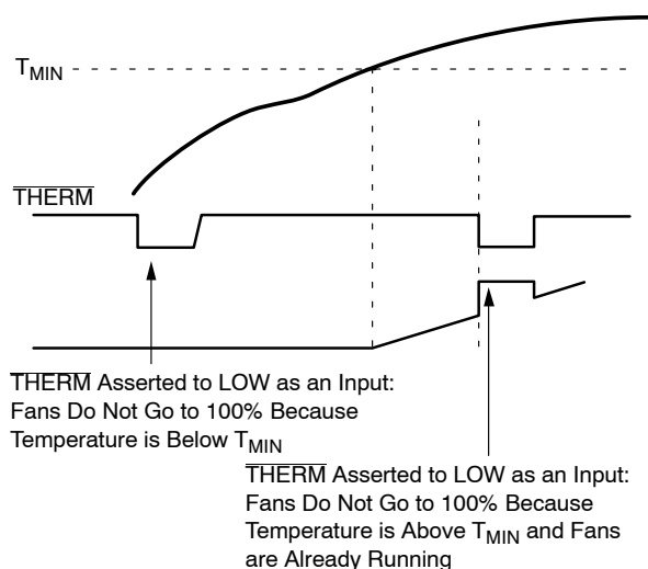
Figure 29. Asserting THERM Low as an Input in Automatic Fan Speed Control Mode
