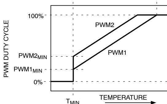
Figure 58. Operating Two Fans from a Single Temperature Channel
