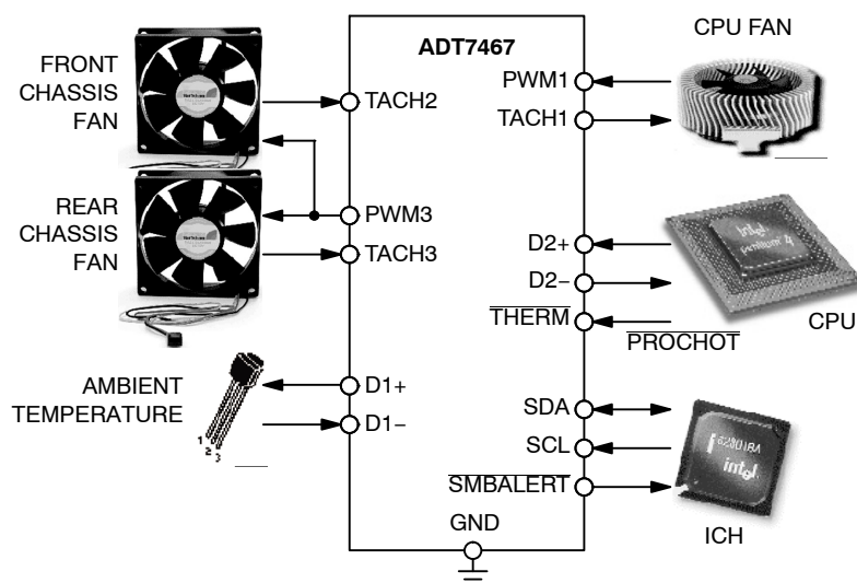
Figure 14. ADT7467 Implementation
