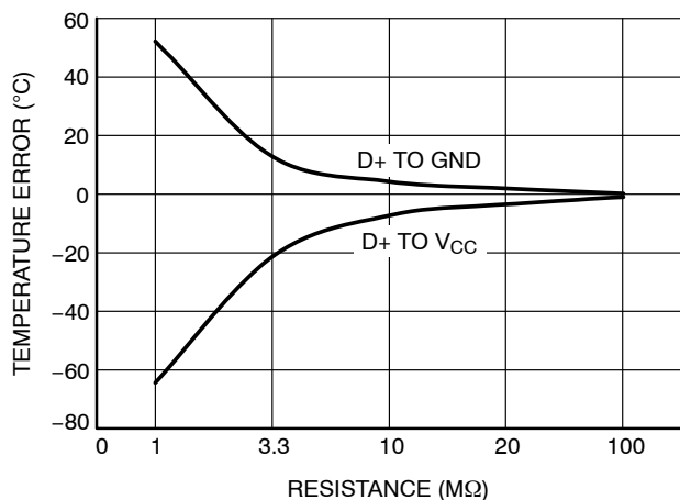
Figure 7. Temperature Error vs. PCB Resistance
