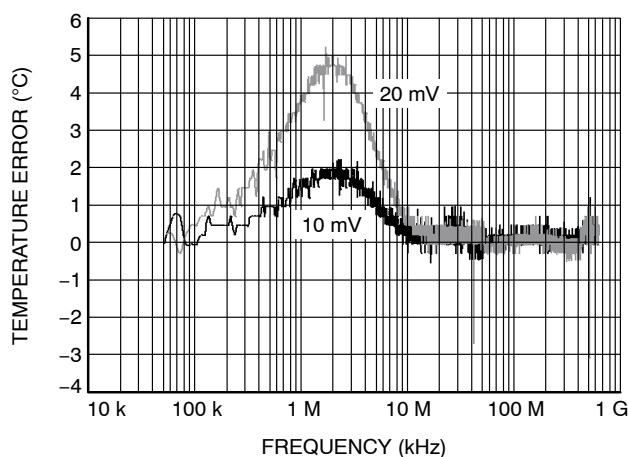
Figure 6. Remote Temperature Error vs. Differential Mode Noise Frequency
