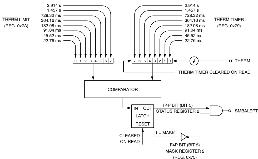
Figure 31. Functional Diagram of \overline{\text{THERM}} Monitoring Circuitry
