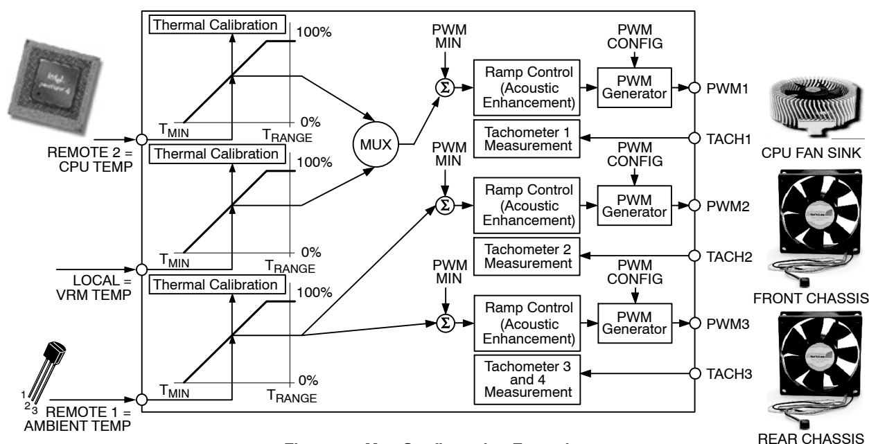
Figure 55. Mux Configuration Example
