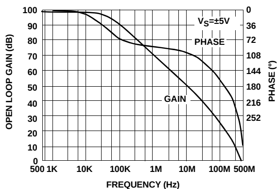
FIGURE 11. OPEN LOOP GAIN AND PHASE vs FREQUENCY
