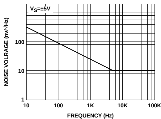
FIGURE 10. EQUIVALENT INPUT VOLTAGE NOISE vs FREQUENCY
