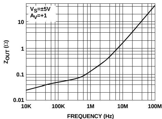
FIGURE 12. Z_{OUT} vs FREQUENCY
