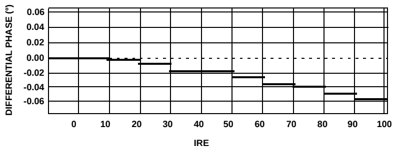
FIGURE 28. DIFFERENTIAL PHASE (°)
