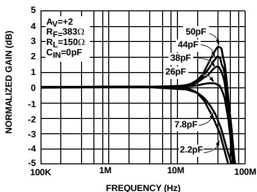
FIGURE 24. GAIN vs FREQUENCY FOR VARIOUS C_L
