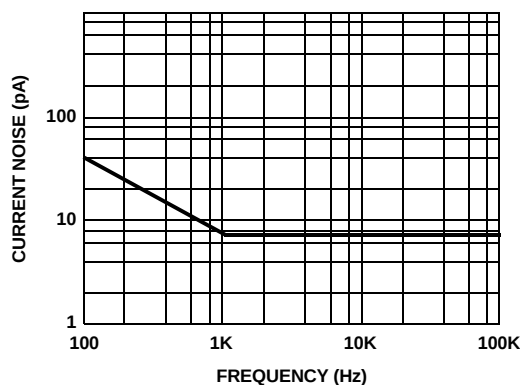
FIGURE 20. CURRENT NOISE
