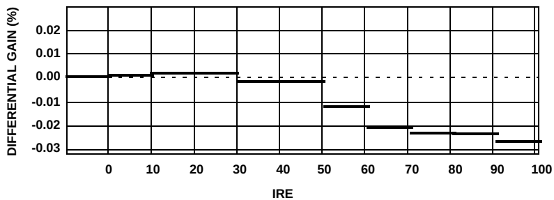
FIGURE 27. DIFFERENTIAL GAIN (%)
