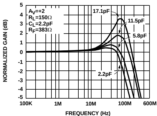
FIGURE 3. GAIN vs FREQUENCY FOR VARIOUS C_{IN}
