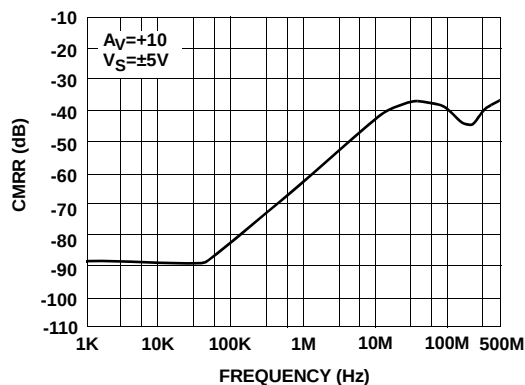
FIGURE 14. CMRR vs FREQUENCY
