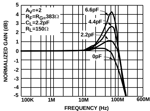
FIGURE 4. GAIN vs FREQUENCY FOR VARIOUS C_{IN}
