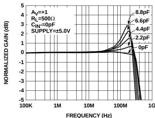
FIGURE 2. GAIN vs FREQUENCY FOR VARIOUS C_L
