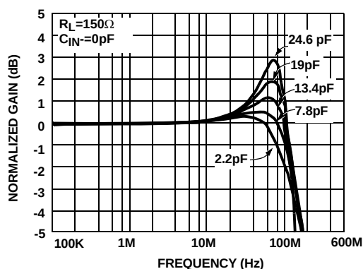
FIGURE 22. GAIN vs FREQUENCY FOR VARIOUS C_L
