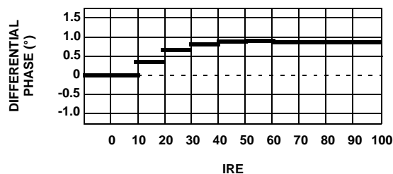
FIGURE 36. DIFFERENTIAL PHASE
