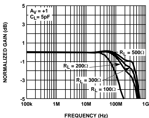
FIGURE 3. EL5150 GAIN vs FREQUENCY FOR VARIOUS R_L
