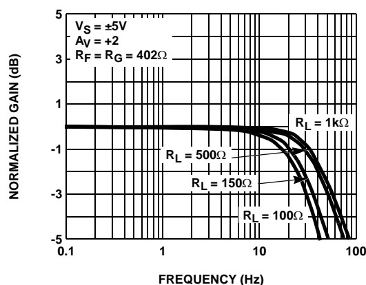
FIGURE 4. EL5150 GAIN vs FREQUENCY FOR VARIOUS R_L
