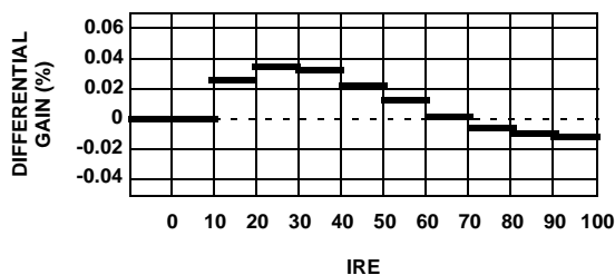
FIGURE 35. DIFFERENTIAL GAIN
