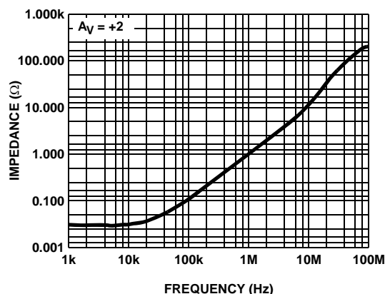
FIGURE 20. OUTPUT IMPEDANCE
