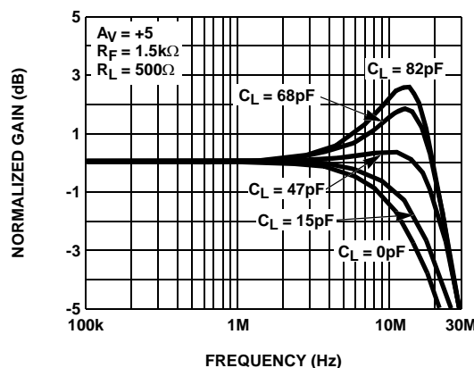
FIGURE 8. EL5150 GAIN vs FREQUENCY FOR VARIOUS C_L
