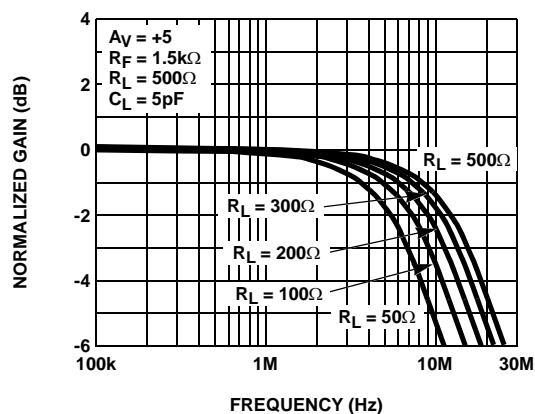
FIGURE 12. EL5250 GAIN vs FREQUENCY FOR VARIOUS R_L
