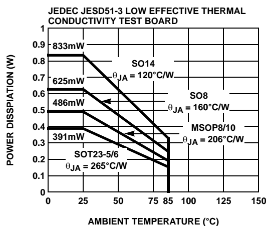
FIGURE 40. PACKAGE POWER DISSIPATION vs AMBIENT TEMPERATURE
