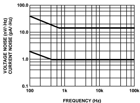
FIGURE 24. VOLTAGE + CURRENT NOISE vs FREQUENCY
