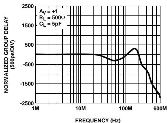
FIGURE 22. GROUP DELAY
