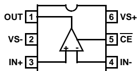
EL5150 (6 LD SOT-23) TOP VIEW
