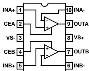
EL5250 (10 LD MSOP) TOP VIEW
