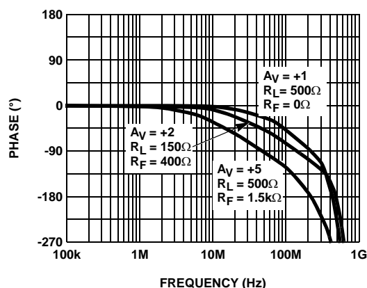
FIGURE 2. PHASE vs FREQUENCY FOR VARIOUS GAINS
