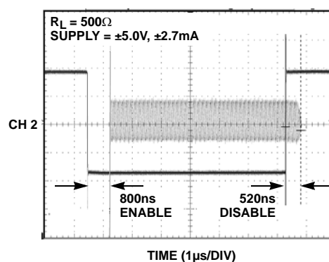
FIGURE 34. EL5250 ENABLE/DISABLE
