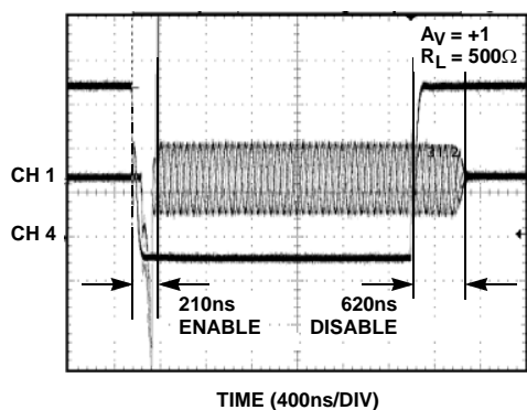
FIGURE 33. EL5150 ENABLE/DISABLE
