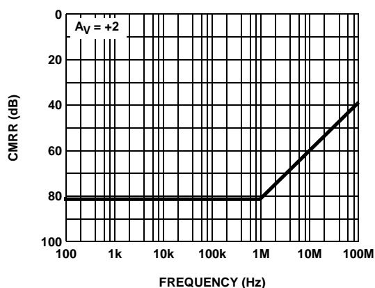
FIGURE 21. CMRR
