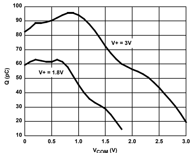
FIGURE 10. CHARGE INJECTION vs SWITCH VOLTAGE
