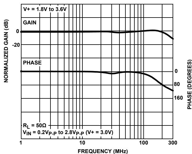
FIGURE 14. FREQUENCY RESPONSE
