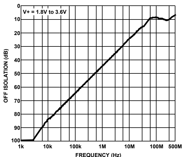
FIGURE 15. OFF ISOLATION
