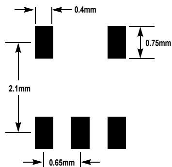
TYPICAL RECOMMENDED LAND PATTERN
