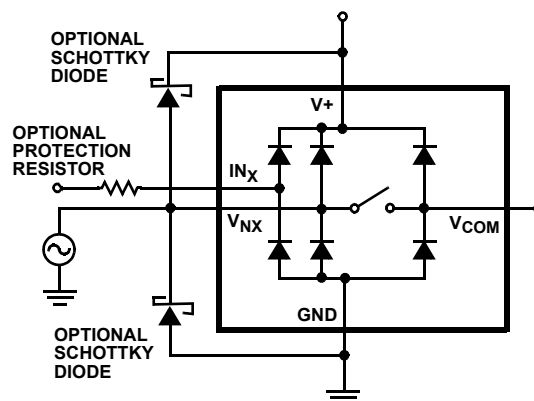
FIGURE 6. OVERVOLTAGE PROTECTION
