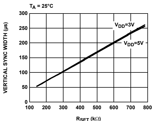
FIGURE 5. VERTICAL SYNC WIDTH vs R_{SET}
