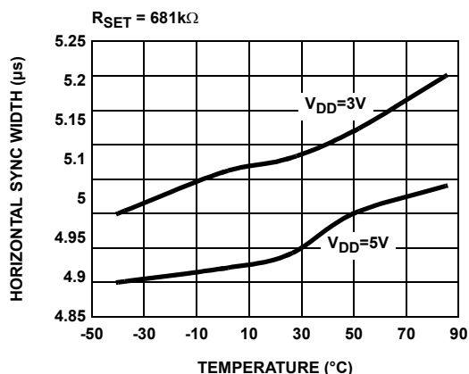
FIGURE 7. HORIZONTAL SYNC WIDTH vs TEMPERATURE
