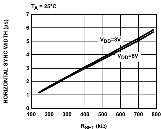
FIGURE 3. HORIZONTAL SYNC WIDTH vs R_{SET}
