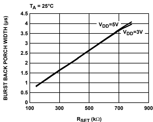
FIGURE 4. BURST/BACK PORCH WIDTH vs R_{SET}
