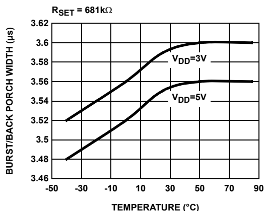
FIGURE 8. BURST/BACK PORCH WIDTH vs TEMPERATURE
