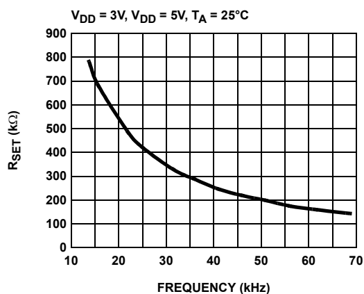
FIGURE 1. R_{SET} vs HORIZONTAL FREQUENCY
