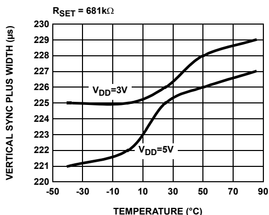
FIGURE 9. VERTICAL SYNC PULSE WIDTH vs TEMPERATURE
