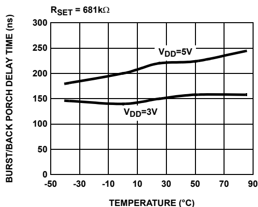
FIGURE 6. BURST/BACK PORCH DELAY vs TEMPERATURE
