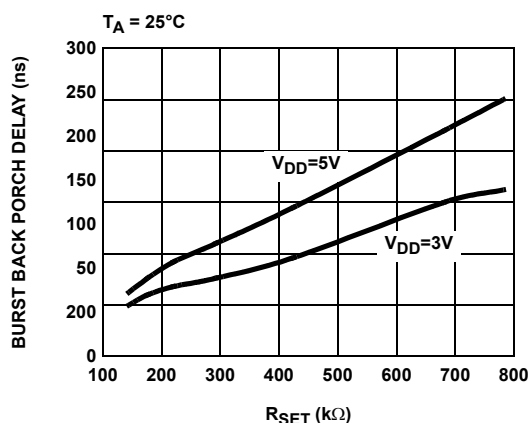
FIGURE 2. BURST/BACK PORCH DELAY vs R_{SET}
