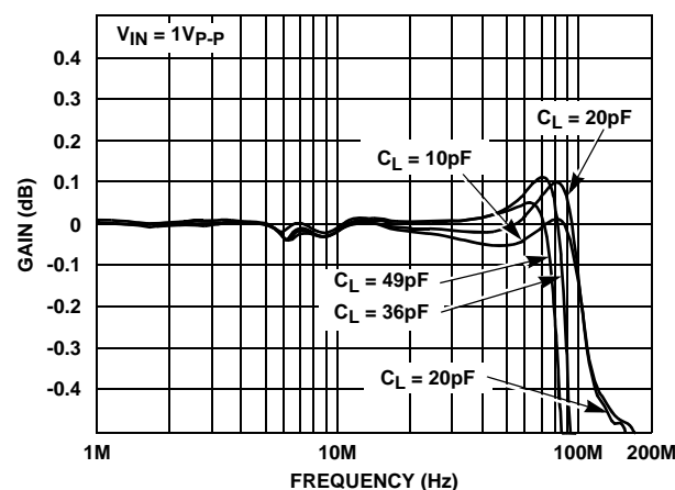
FIGURE 6. GAIN FLATNESS
