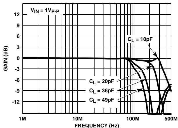
FIGURE 5. FREQUENCY RESPONSE
