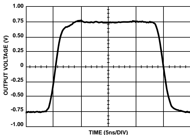
FIGURE 3. LARGE SIGNAL PULSE RESPONSE
