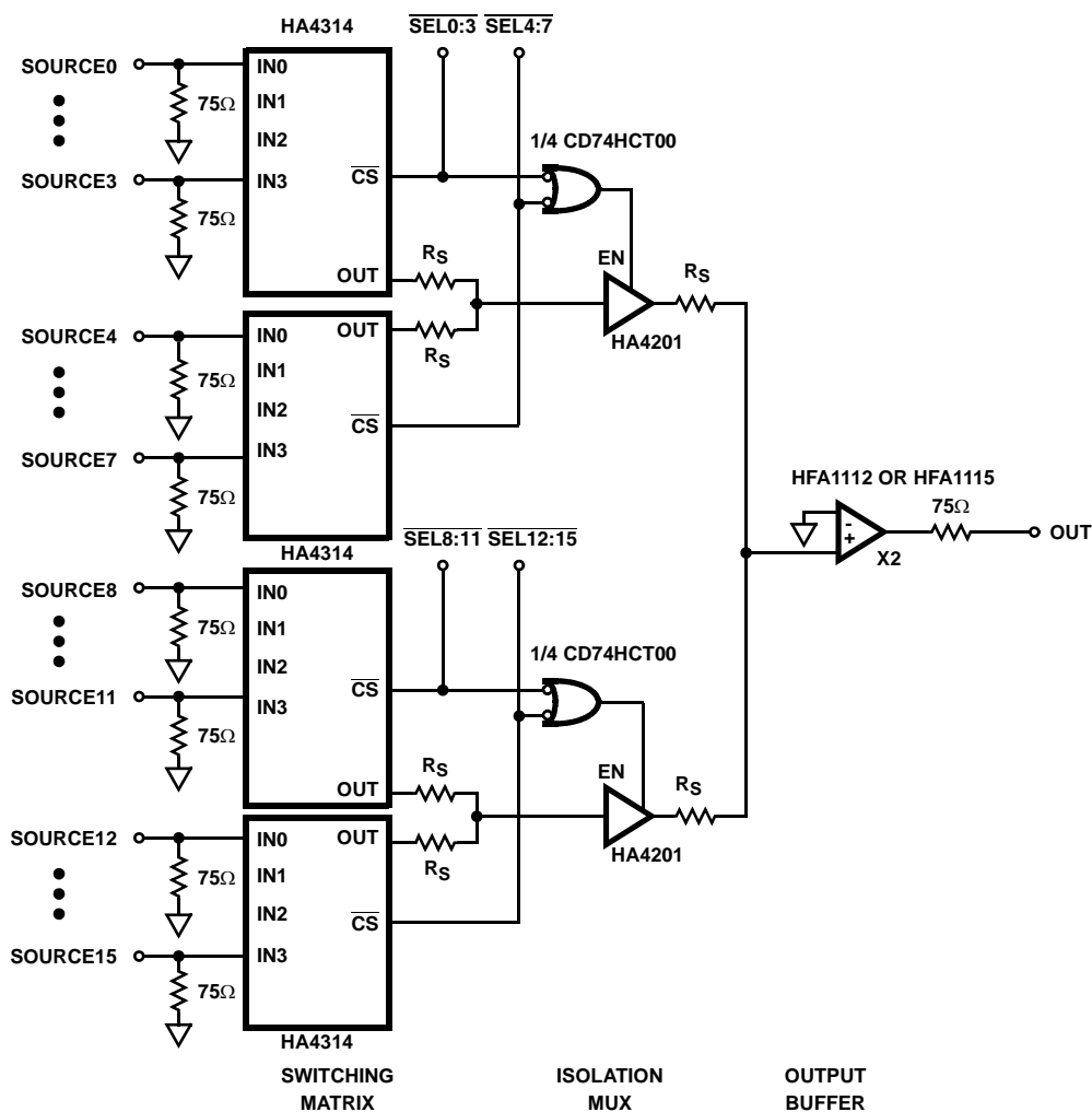
FIGURE 2. 16x1 SWITCHER APPLICATION
