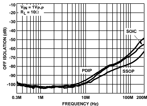
FIGURE 8. ALL HOSTILE OFF ISOLATION
