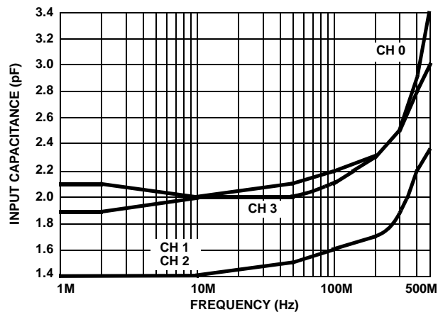
FIGURE 10. INPUT CAPACITANCE vs FREQUENCY
