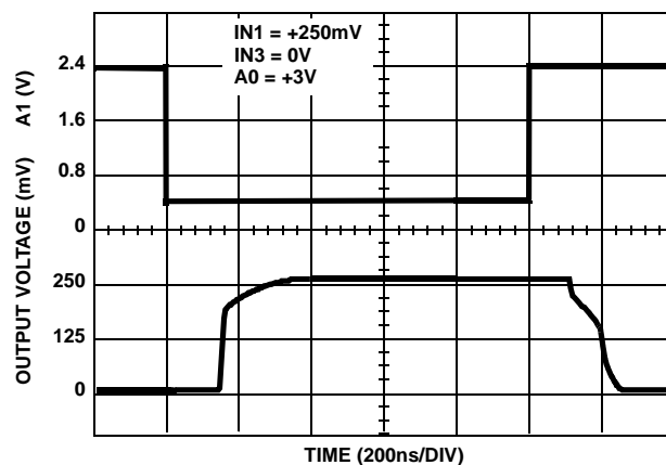
FIGURE 4. CHANNEL-TO-CHANNEL SWITCHING RESPONSE
