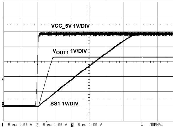
FIGURE 13. SOFT-START OPERATION
