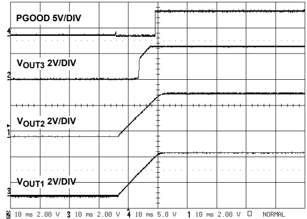
FIGURE 4. SOFT-START WAVEFORMS WITH PGOOD
