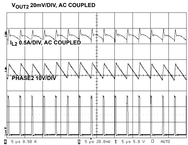
FIGURE 6. PWM2 WAVEFORMS
