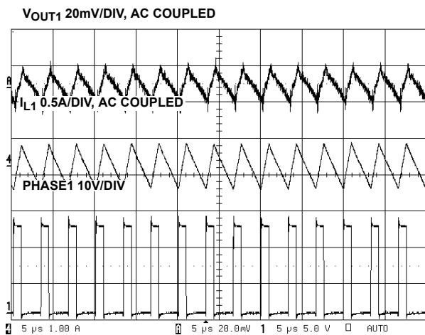
FIGURE 5. PWM1 WAVEFORMS
