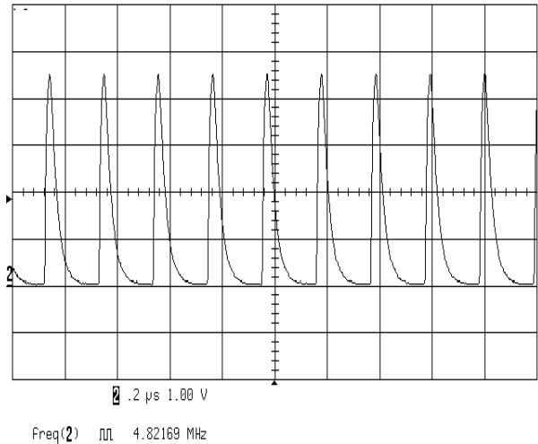
FIGURE 18. SYNC WAVEFORM
