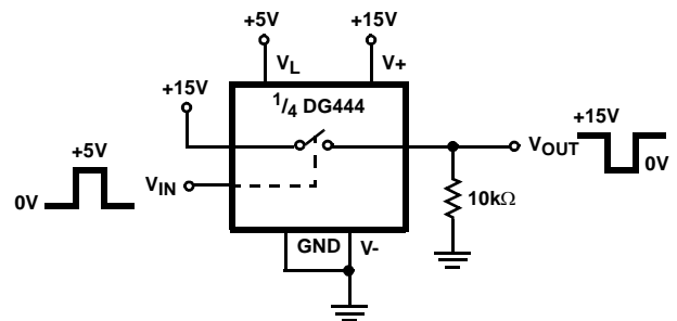
FIGURE 7. LEVEL SHIFTER
