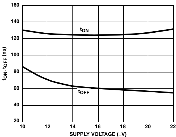
FIGURE 18. SWITCHING TIME vs POWER SUPPLY VOLTAGE (DG444)
