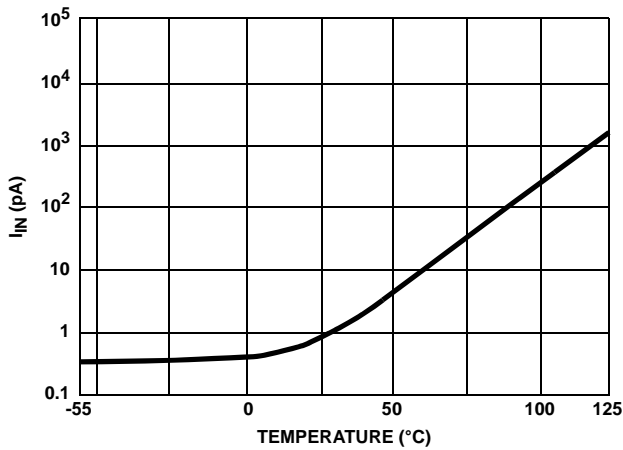
FIGURE 10. INPUT CURRENT vs TEMPERATURE
