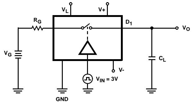
FIGURE 2B. TEST CIRCUIT
