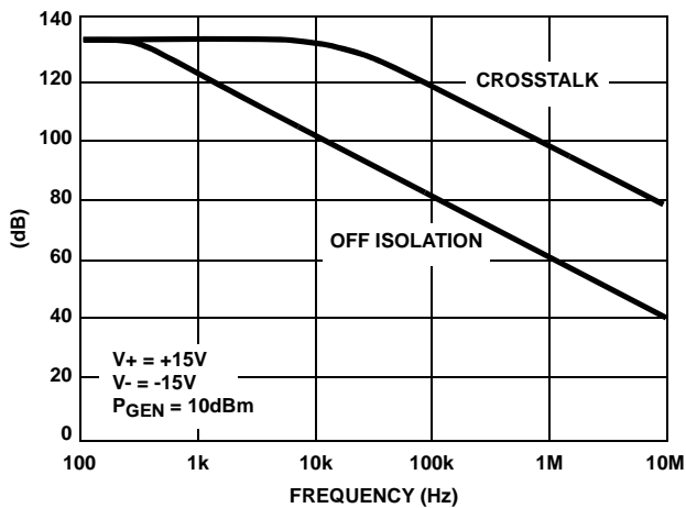
FIGURE 12. CROSSTALK REJECTION AND OFF ISOLATION vs FREQUENCY
