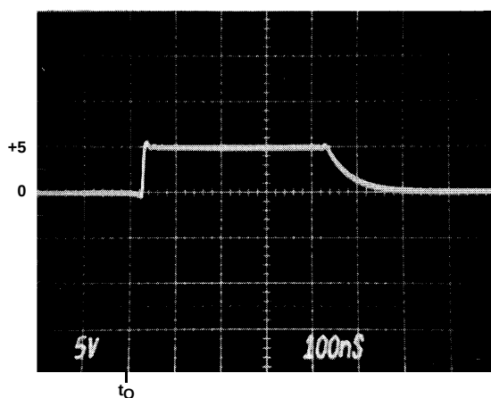
FIGURE 2C. V_{IN} = +5V
