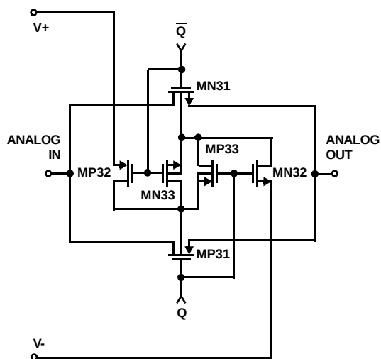
SWITCH CELL
