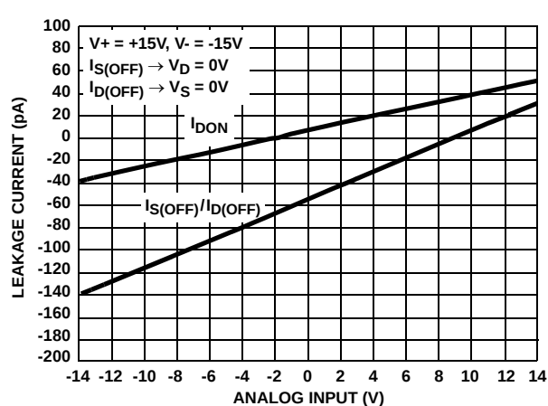
FIGURE 8. LEAKAGE CURRENT vs ANALOG INPUT VOLTAGE
