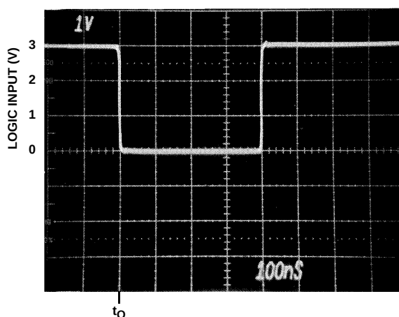
FIGURE 2A. LOGIC INPUT WAVEFORM
