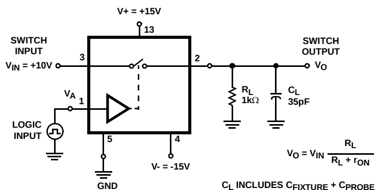
FIGURE 1C. TEST CIRCUIT
