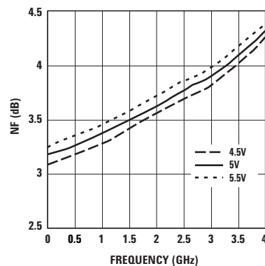
Figure 4. Noise Figure vs. Frequency and Voltage.
