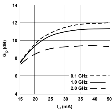
Figure 2. Power Gain vs. Current.
