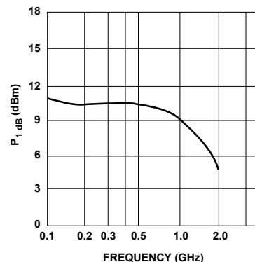
Figure 3. Output Power at 1 dB Gain Compression vs. Frequency, I_d = 35 \text{ mA} .
