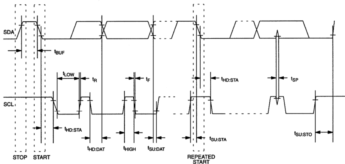
Figure 3. TIMING DIAGRAM
