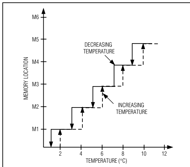
Figure 4. Look-Up Table Hysteresis
