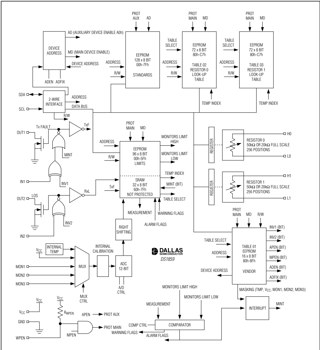
Figure 1. Block Diagram
