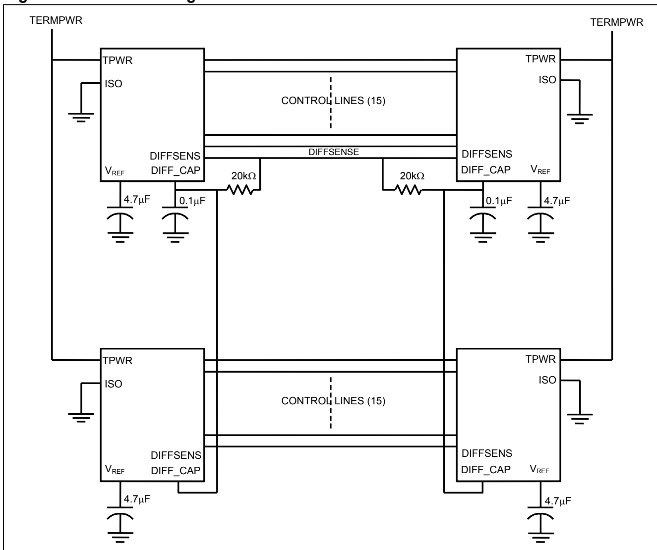
Figure 2. SCSI Bus Configuration
