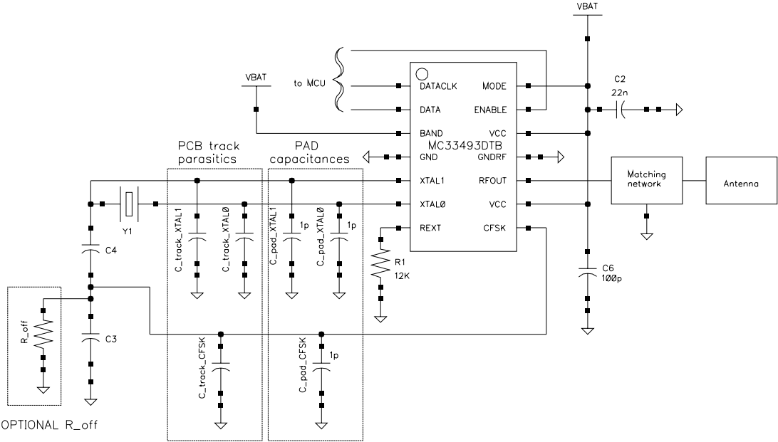
Figure 16. Crystal Load Capacitance Contributors Schematic
