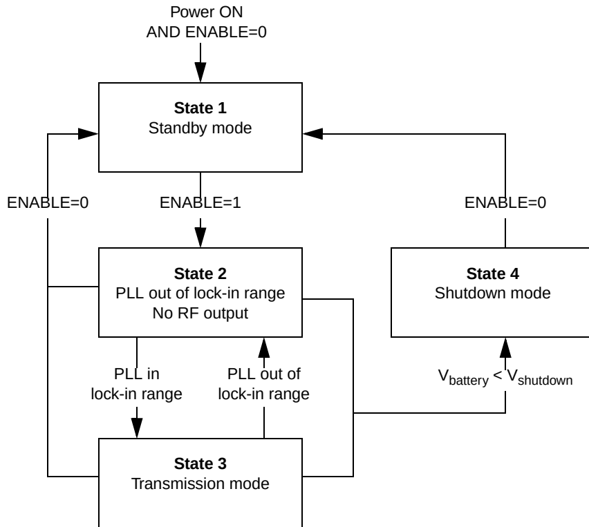
Figure 3. State machine
