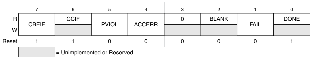
Figure 21-10. Flash Status Register (FSTAT)
