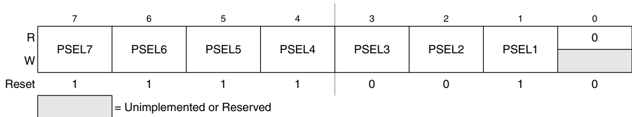
Figure 5-4. Highest Priority I Interrupt Register (HPRIO)
