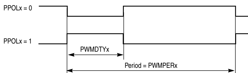
Figure 12-36. PWM Left Aligned Output Waveform
