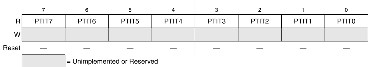
Figure 2-4. Port T Input Register (PTIT)
