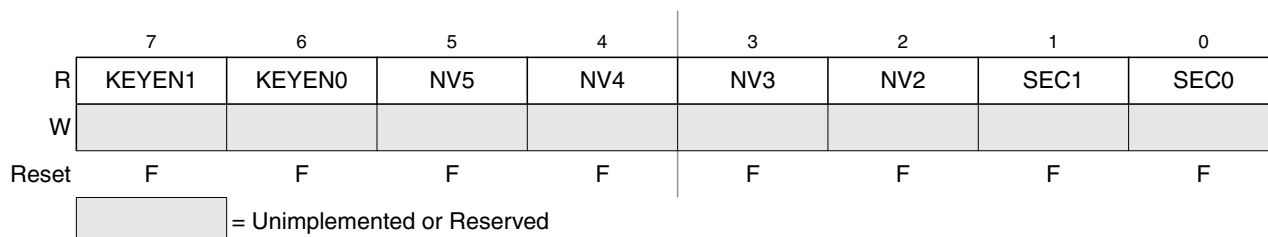
Figure 21-5. Flash Security Register (FSEC)
