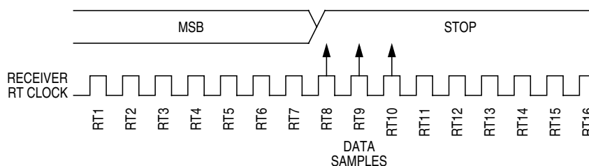
Figure 13-20. Slow Data
