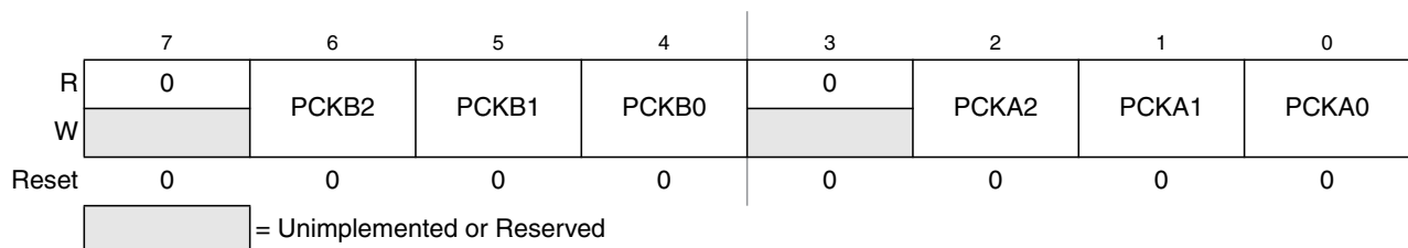
Figure 12-6. PWM Prescaler Clock Select Register (PWMPRCLK)
