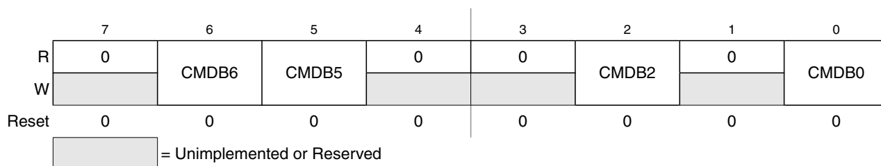
Figure 21-11. Flash Command Register (FCMD)
