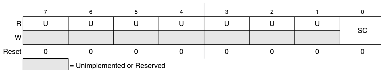
Figure 8-11. ATD Test Register 1 (ATDTEST1)
