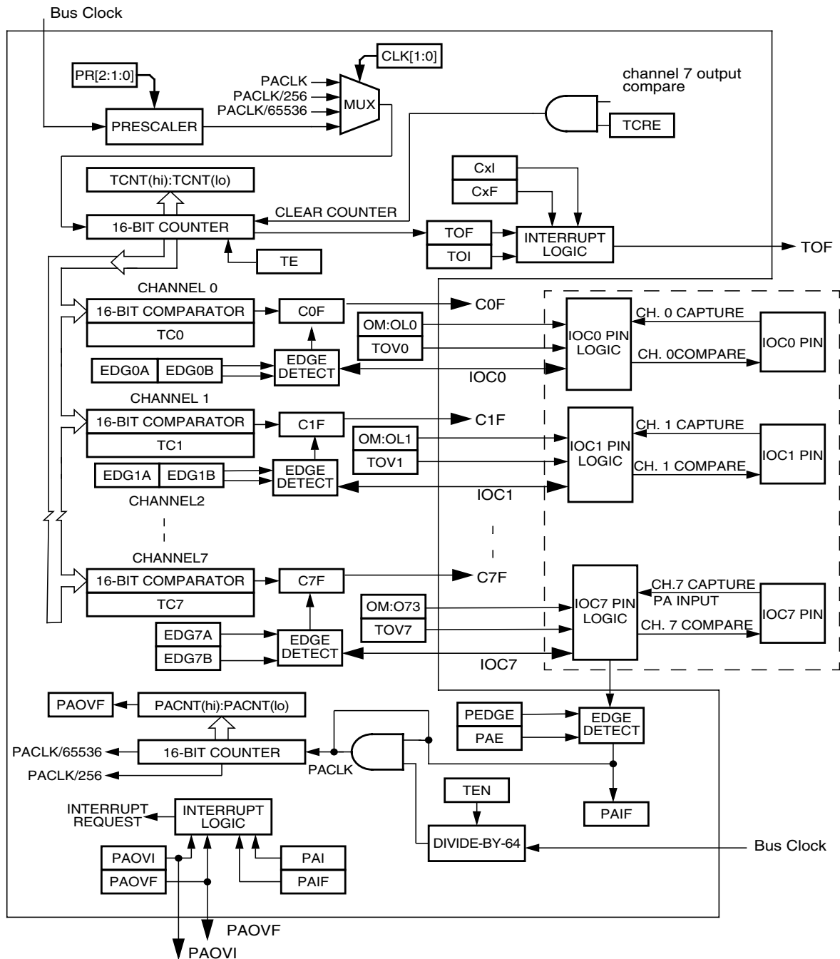
Figure 15-28. Detailed Timer Block Diagram
