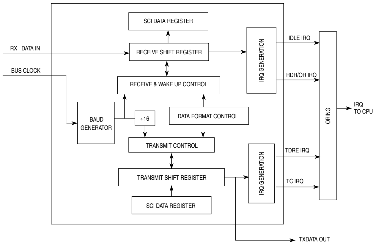
Figure 13-1. SCI Block Diagram
