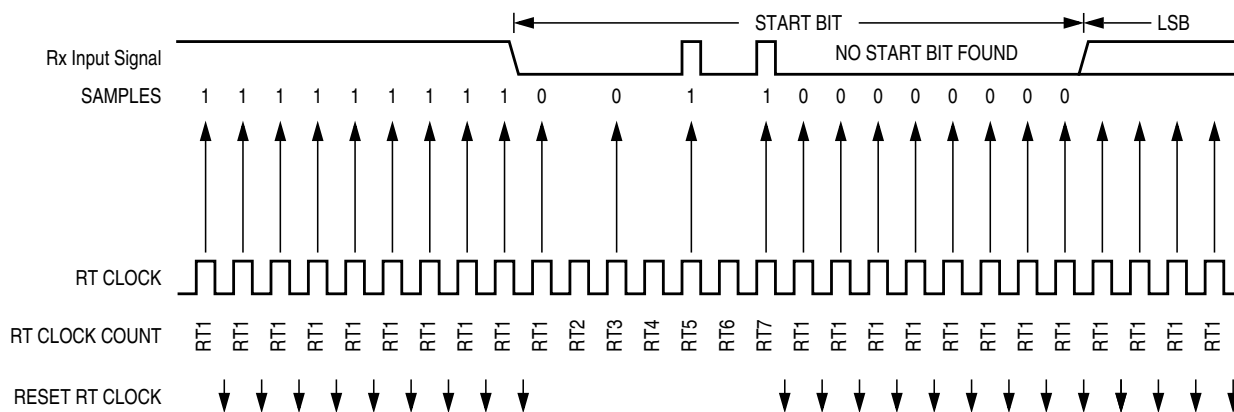
Figure 13-18. Start Bit Search Example 5
