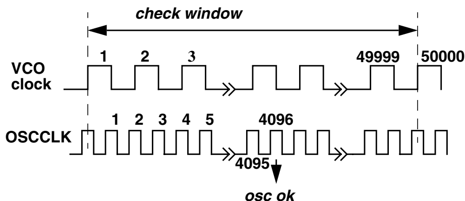
Figure 9-19. Check Window Example
