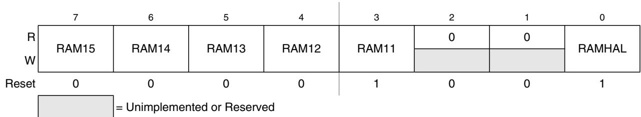
Figure 3-3. Initialization of Internal RAM Position Register (INITRM)
