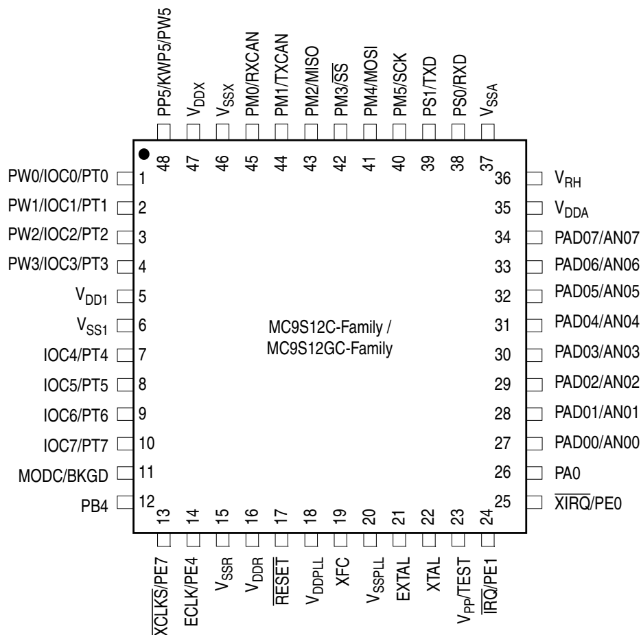
Figure 1-9. Pin Assignments in 48-Pin LQFP
