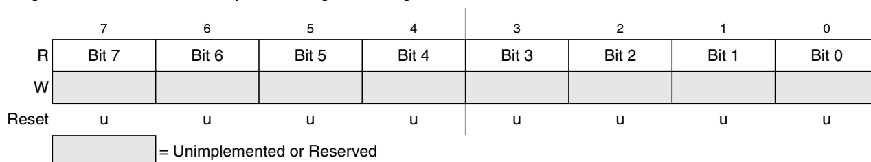
Figure 7-7. Debug Trace Buffer Register Low (DBGTBL)
