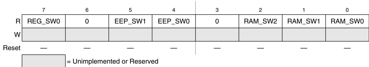
Figure 3-9. Memory Size Register 0 (MEMSIZ0)
