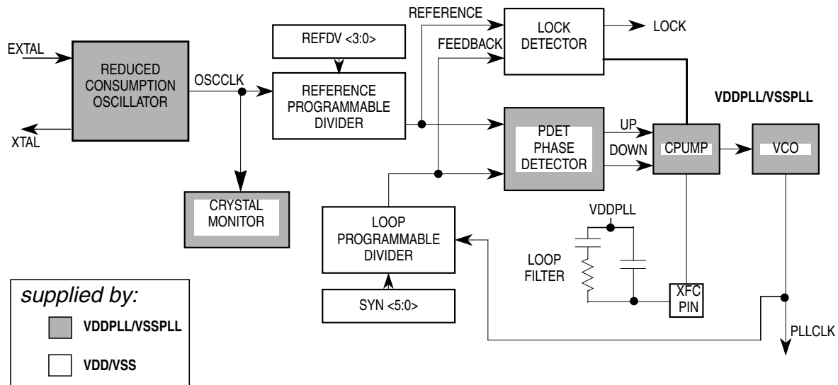
Figure 9-16. PLL Functional Diagram
