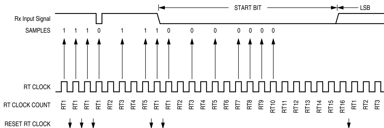
Figure 13-14. Start Bit Search Example 1
