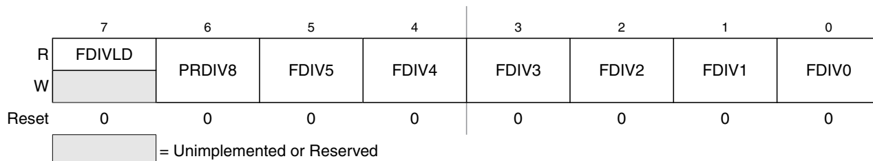
Figure 21-4. Flash Clock Divider Register (FCLKDIV)
