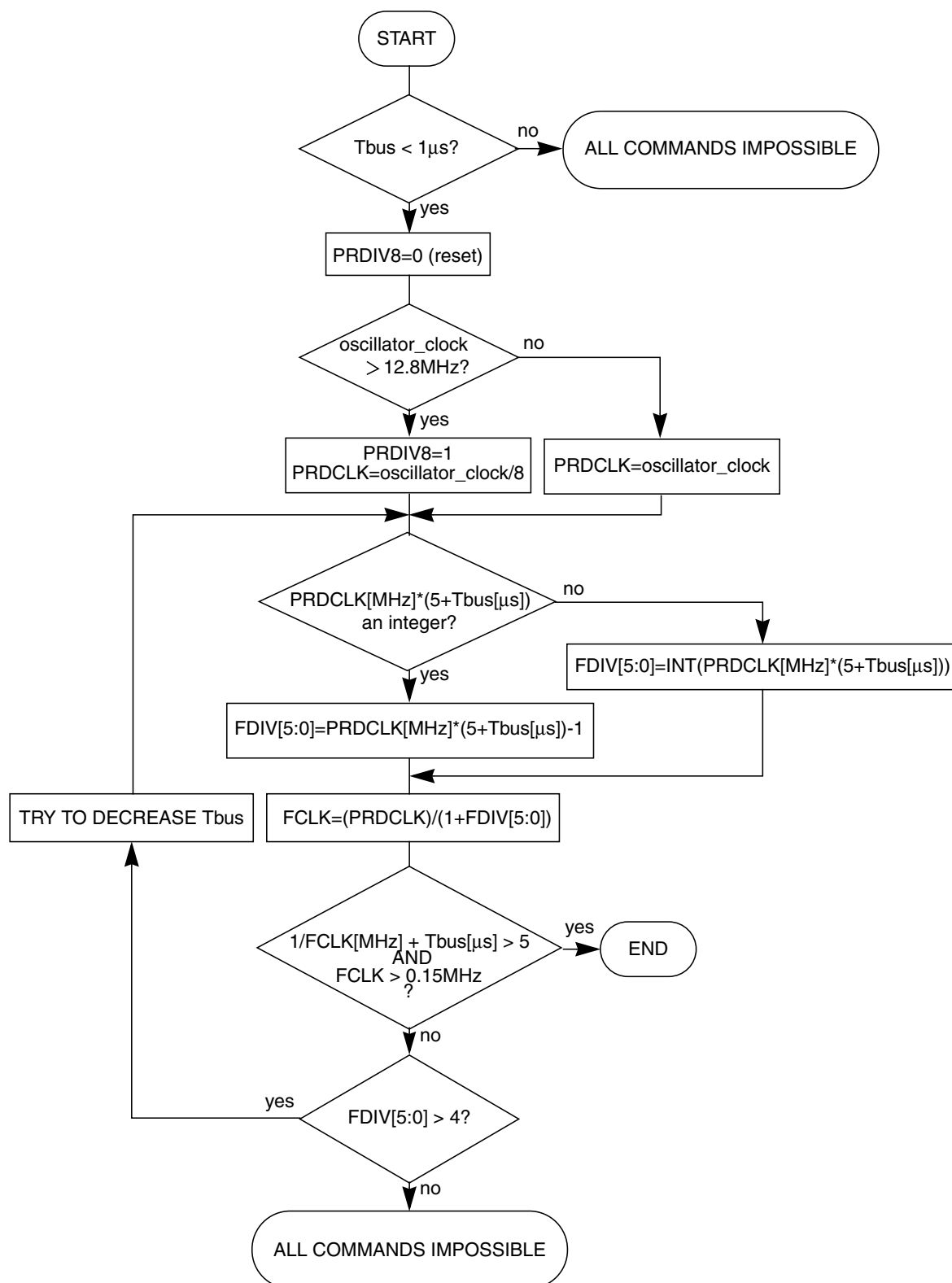
Figure 19-24. PRDIV8 and FDIV Bits Determination Procedure
