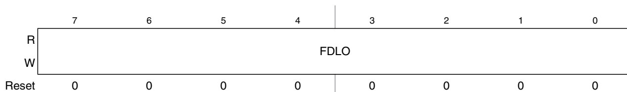
Figure 21-16. Flash Data Low Register (FDATALO)
