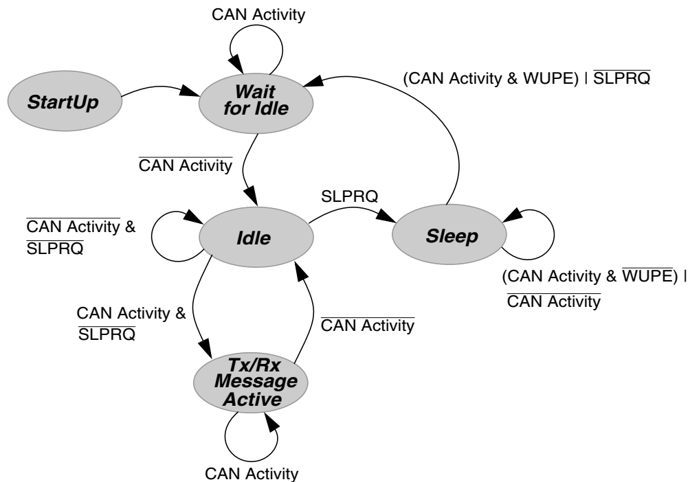
Figure 10-45. Simplified State Transitions for Entering/Leaving Sleep Mode
