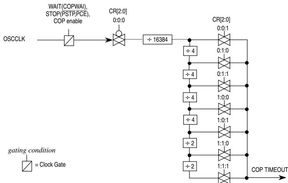
Figure 9-21. Clock Chain for COP
