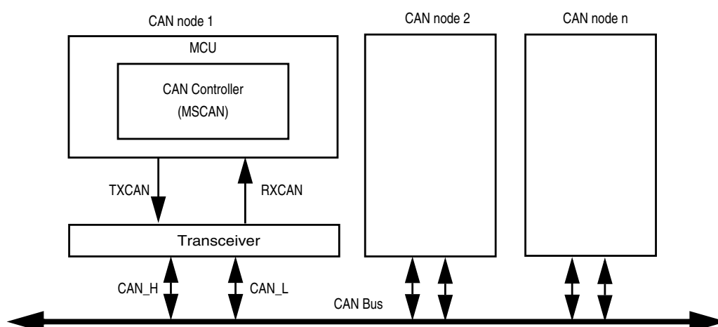
Figure 10-2. CAN System
