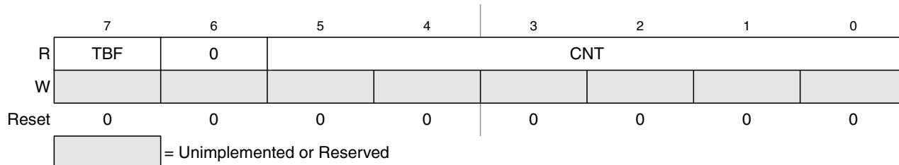
Figure 7-8. Debug Count Register (DBGCNT)
