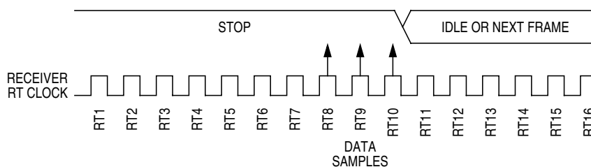
Figure 13-21. Fast Data
