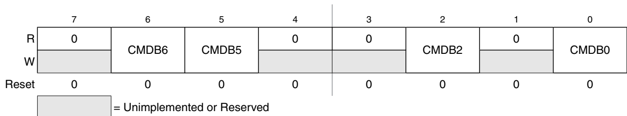
Figure 17-11. Flash Command Register (FCMD)
