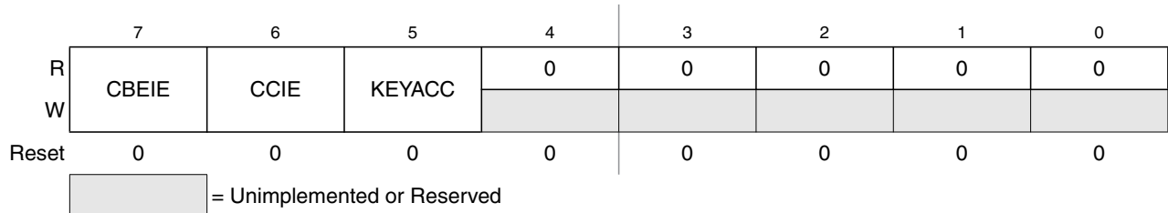
Figure 20-9. Flash Configuration Register (FCNFG)
