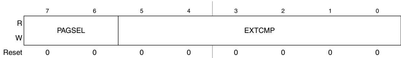
Figure 7-9. Debug Comparator C Extended Register (DBGCCX)
