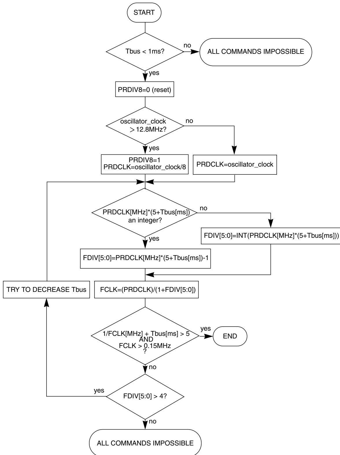
Figure 18-21. PRDIV8 and FDIV Bits Determination Procedure
