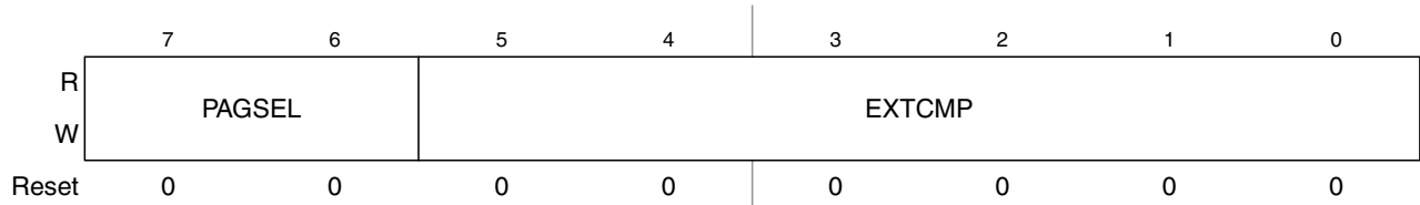
Figure 7-19. Debug Comparator B Extended Register (DBGCBX)
