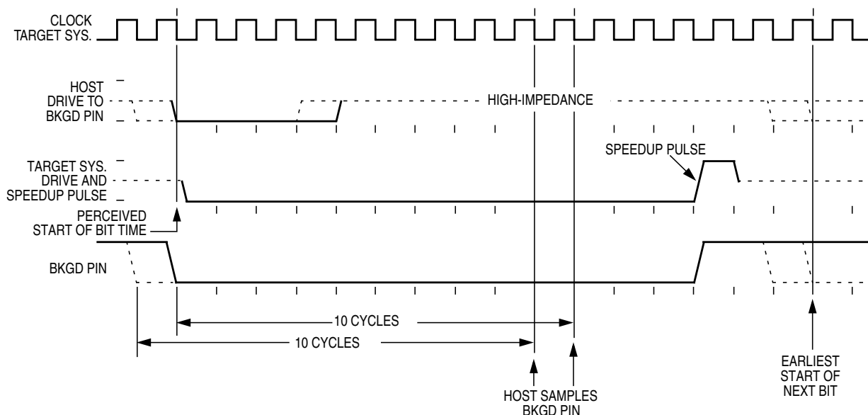
Figure 6-9. BDM Target-to-Host Serial Bit Timing (Logic 0)
