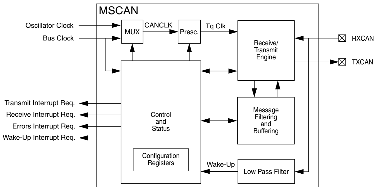
Figure 10-1. MSCAN Block Diagram
