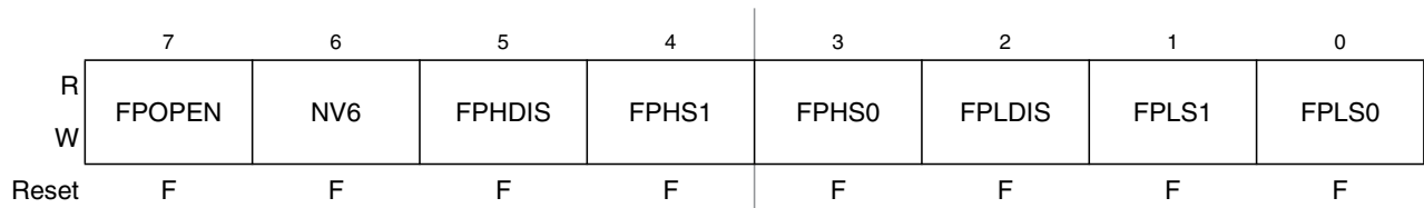
Figure 20-10. Flash Protection Register (FPROT)
