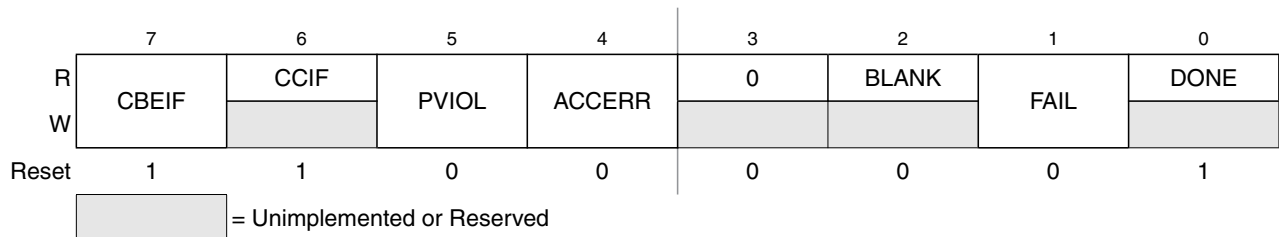
Figure 17-10. Flash Status Register (FSTAT)
