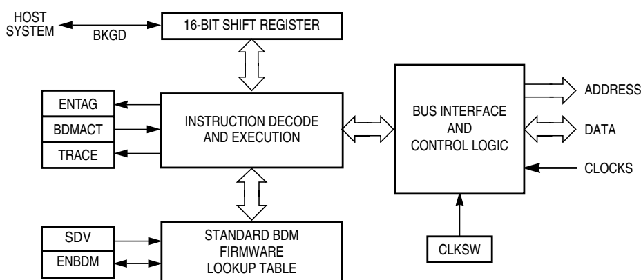
Figure 6-1. BDM Block Diagram
