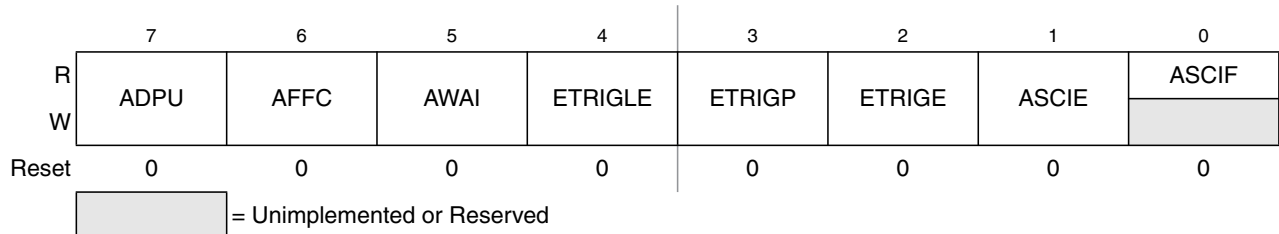
Figure 8-5. ATD Control Register 2 (ATDCTL2)
