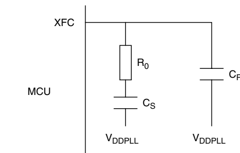
Figure 1-10. PLL Loop Filter Connections
