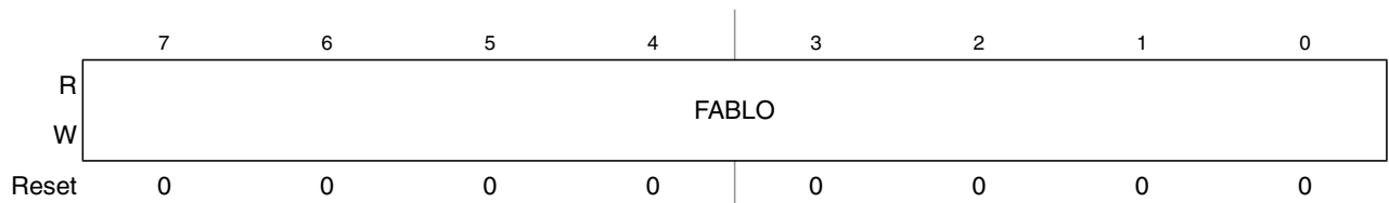
Figure 19-17. Flash Address Low Register (FADDRLO)
