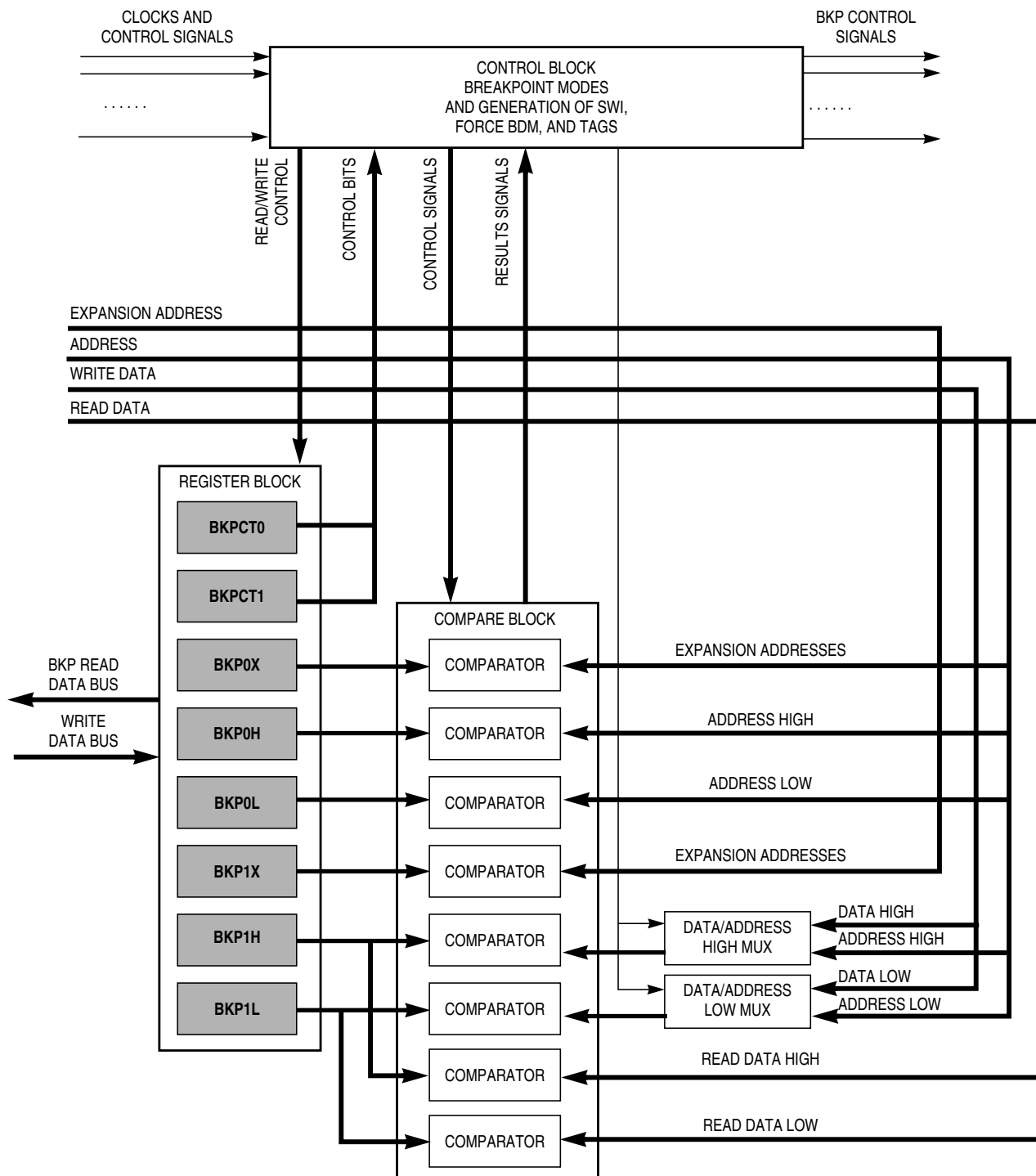
Figure 7-1. DBG Block Diagram in BKP Mode
