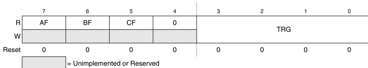
Figure 7-5. Debug Status and Control Register (DBGSC)
