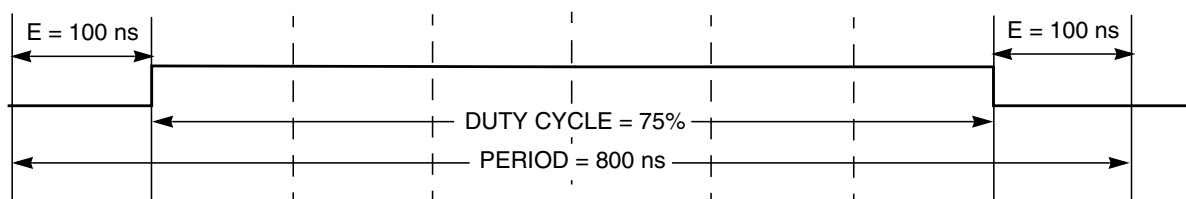
Figure 12-39. PWM Center Aligned Output Example Waveform
