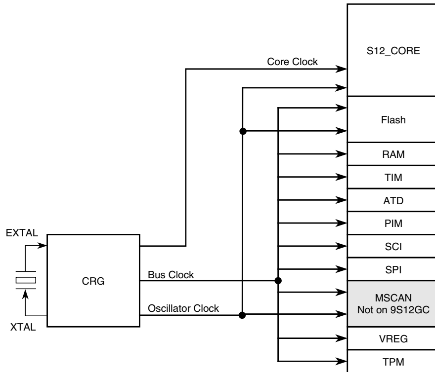
Figure 1-14. Clock Connections
