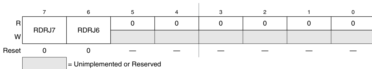
Figure 2-35. Port J Reduced Drive Register (RDRJ)
