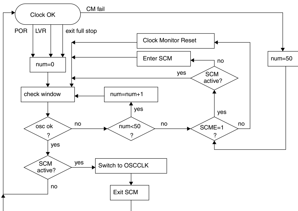
Figure 9-20. Sequence for Clock Quality Check
