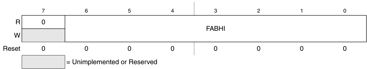
Figure 19-16. Flash Address High Register (FADDRHI)
