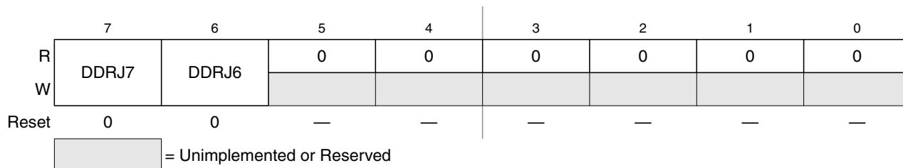
Figure 2-34. Port J Data Direction Register (DDRJ)
