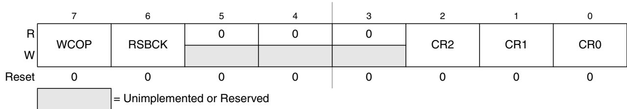
Figure 9-12. CRG COP Control Register (COPCTL)
