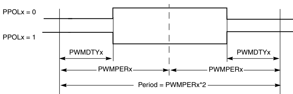
Figure 12-38. PWM Center Aligned Output Waveform
