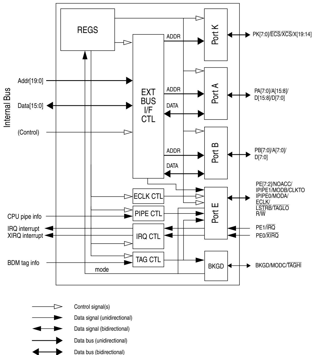
Figure 4-1. MEBI Block Diagram
