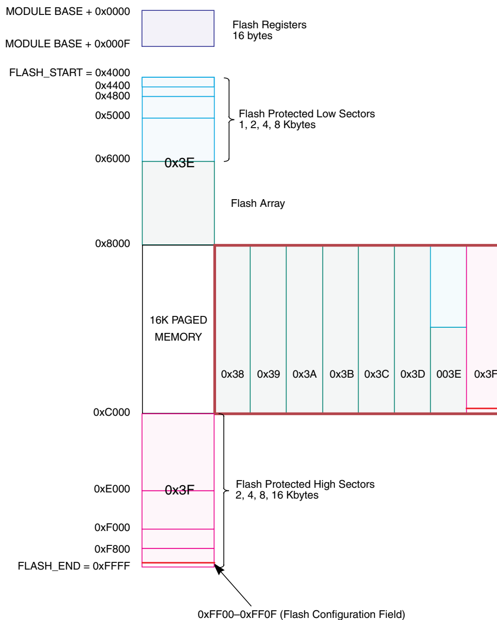
Figure 19-3. Flash Memory Map
