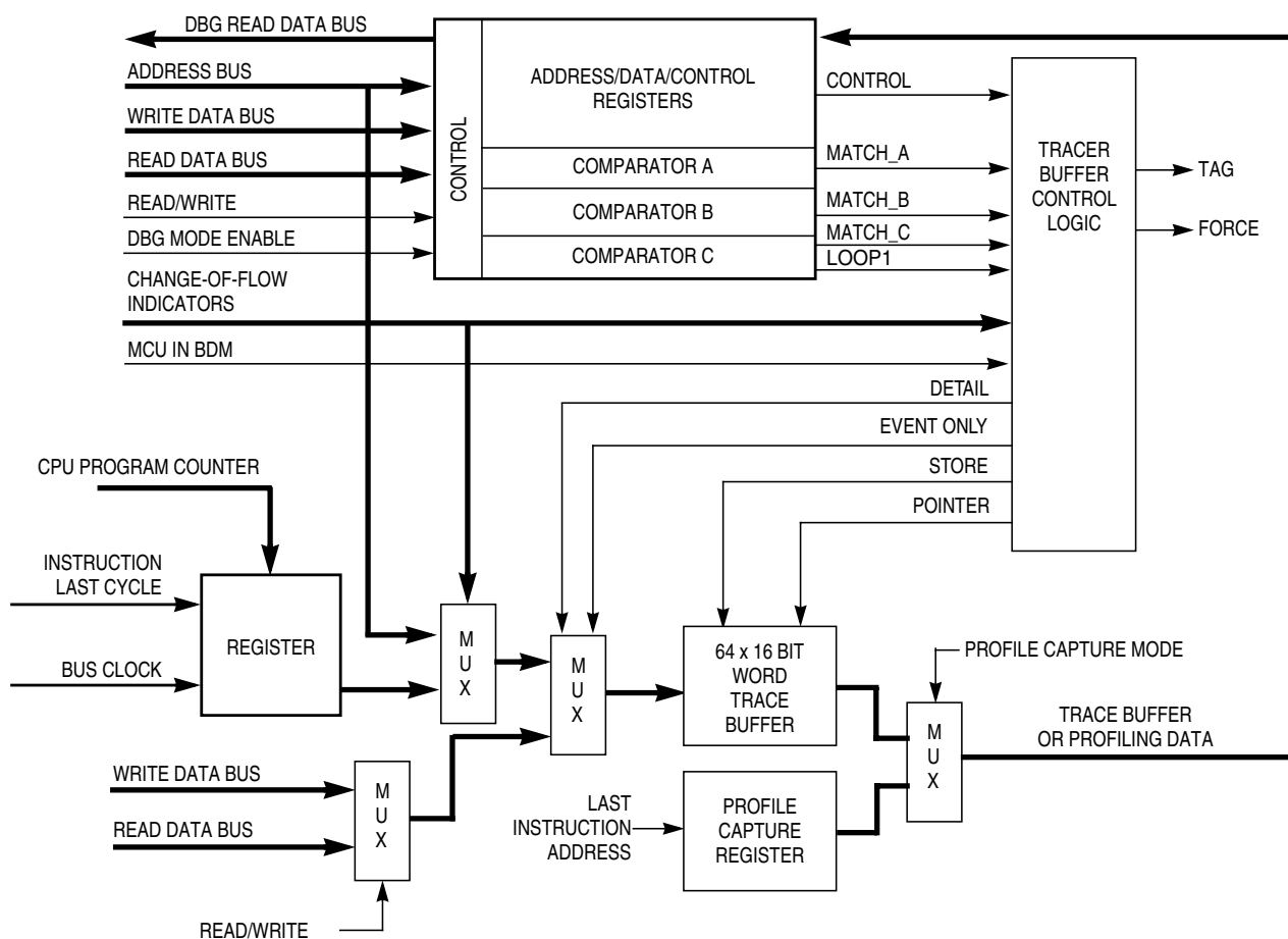
Figure 7-2. DBG Block Diagram in DBG Mode
