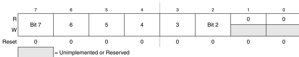
Figure 4-11. Data Direction Register E (DDRE)
