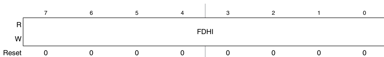
Figure 17-15. Flash Data High Register (FDATAHI)
