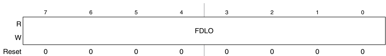
Figure 19-19. Flash Data Low Register (FDATALO)
