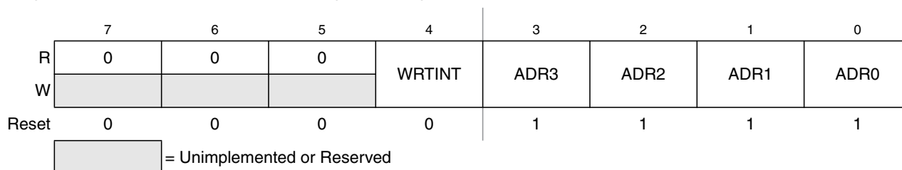
Figure 5-2. Interrupt Test Control Register (ITCR)
