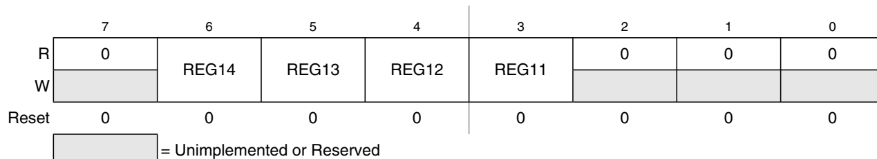
Figure 3-4. Initialization of Internal Registers Position Register (INITRG)
