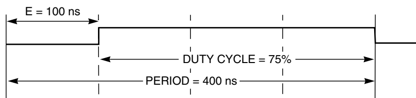
Figure 12-37. PWM Left Aligned Output Example Waveform
