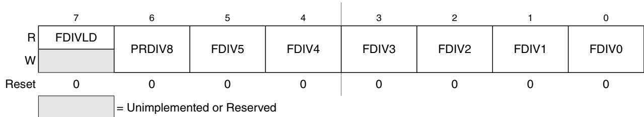
Figure 20-6. Flash Clock Divider Register (FCLKDIV)
