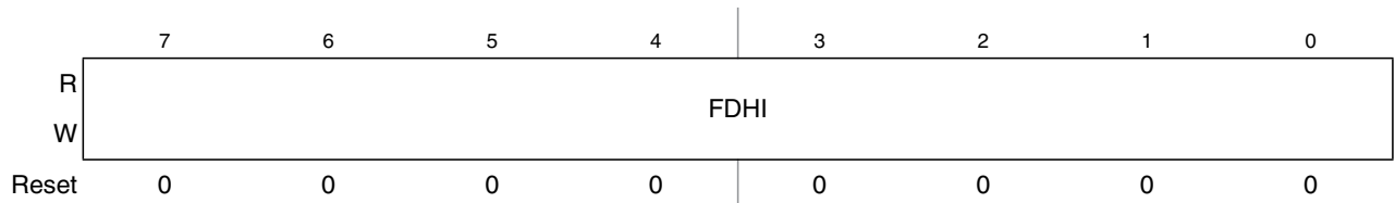
Figure 19-18. Flash Data High Register (FDATAHI)
