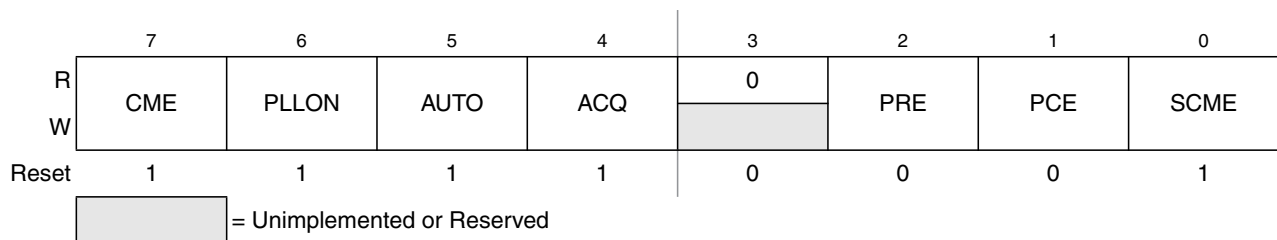
Figure 9-10. CRG PLL Control Register (PLLCTL)
