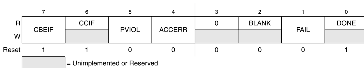
Figure 20-12. Flash Status Register (FSTAT)
