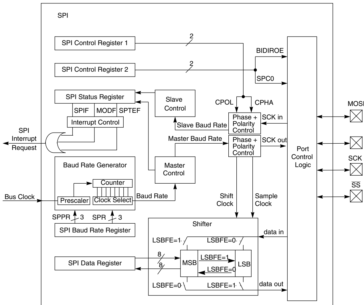
Figure 14-1. SPI Block Diagram
