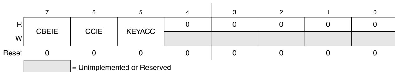
Figure 19-9. Flash Configuration Register (FCNFG)
