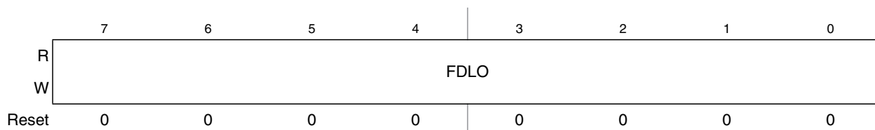
Figure 20-18. Flash Data Low Register (FDATALO)
