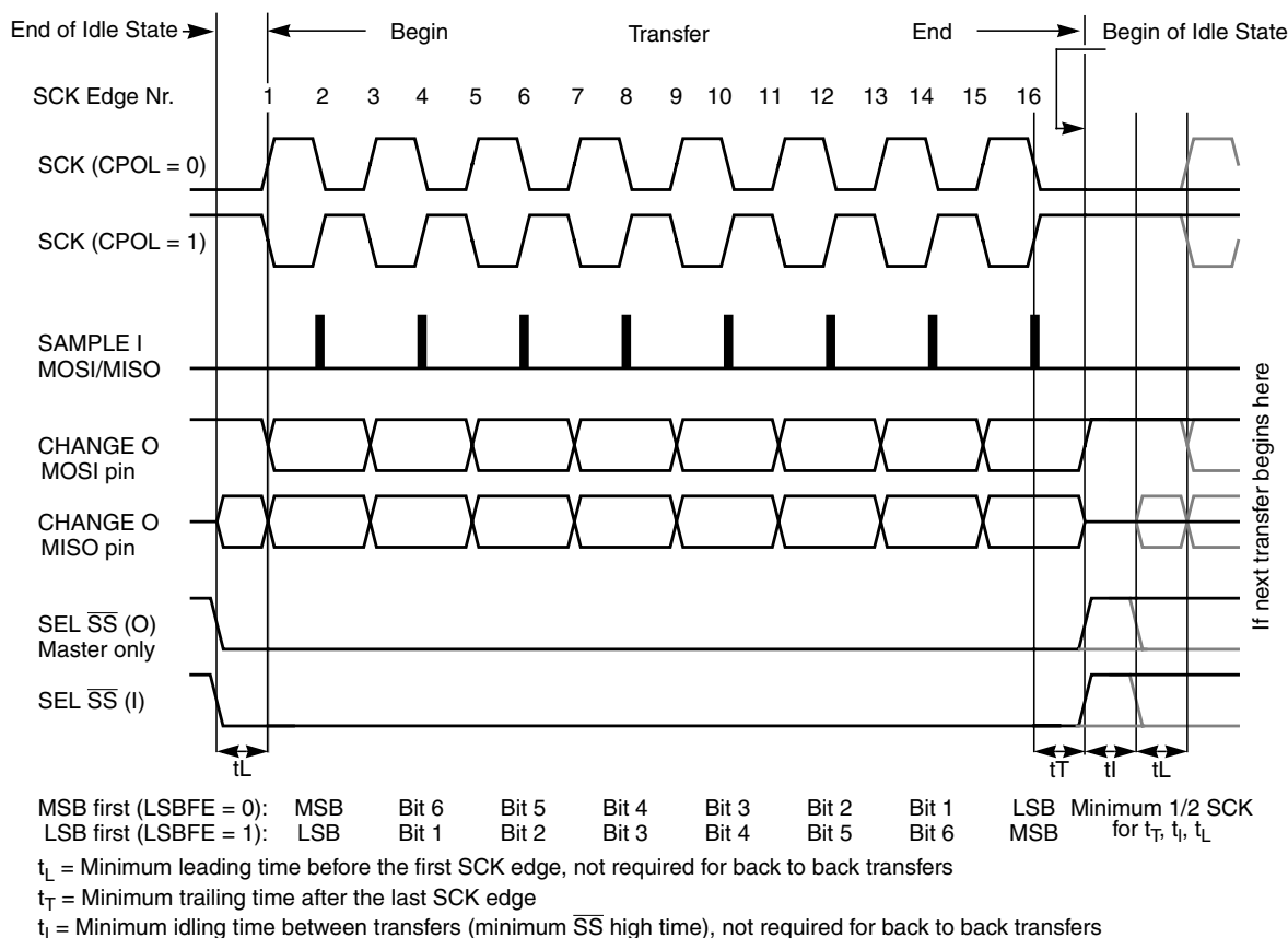
Figure 14-10. SPI Clock Format 1 (CPHA = 1)
