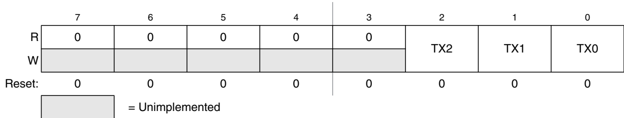
Figure 10-14. MSCAN Transmit Buffer Selection Register (CANTBSEL)
