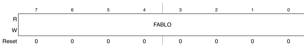
Figure 20-16. Flash Address Low Register (FADDRLO)
