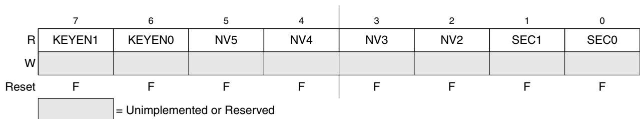
Figure 19-7. Flash Security Register (FSEC)
