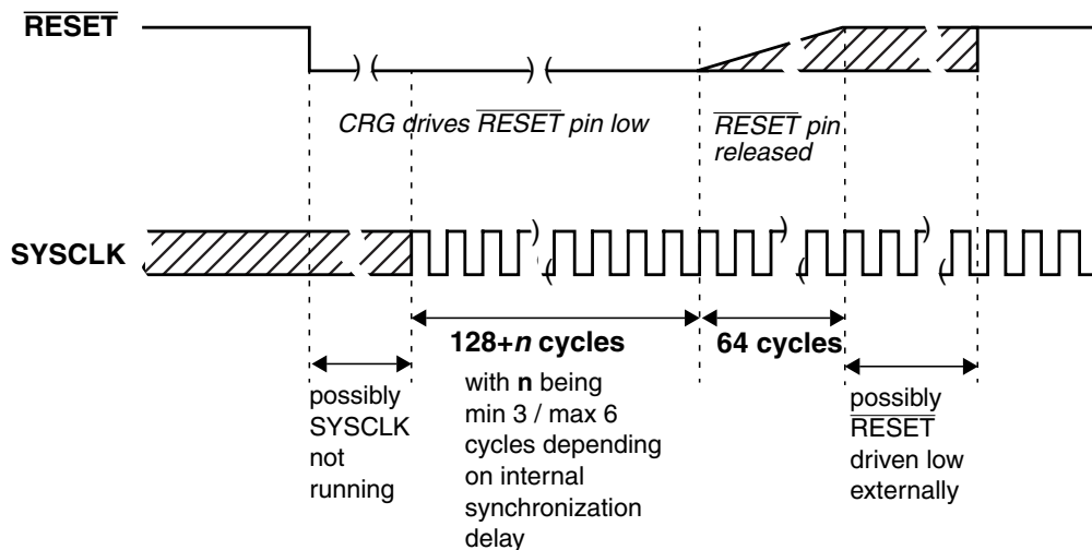
Figure 9-25. \overline{\text{RESET}} Timing
