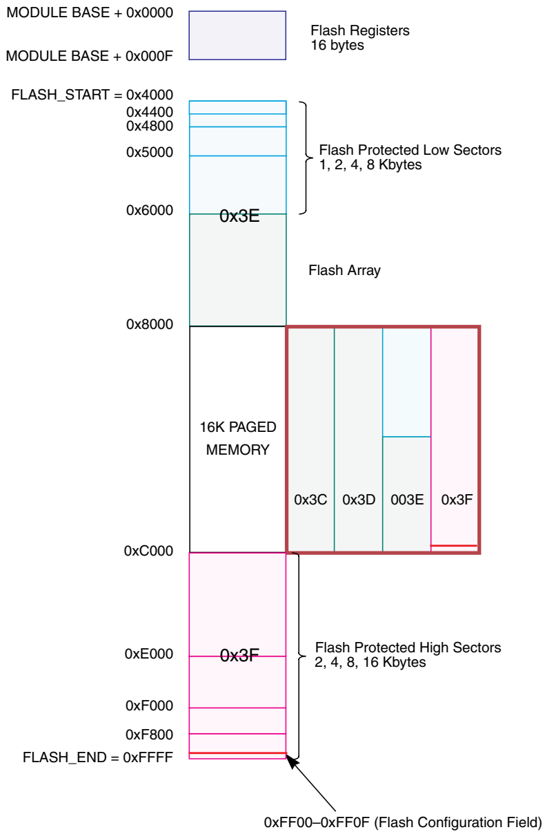
Figure 19-4. Flash Memory Map
