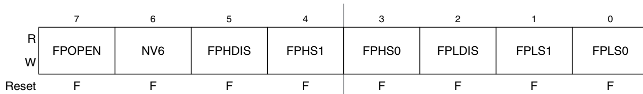
Figure 19-10. Flash Protection Register (FPROT)
