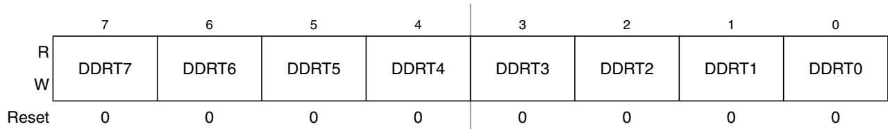
Figure 2-5. Port T Data Direction Register (DDRT)
