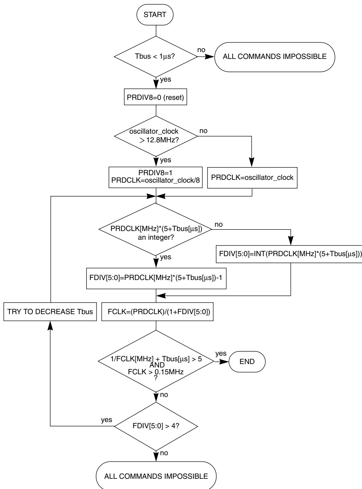
Figure 17-21. PRDIV8 and FDIV Bits Determination Procedure
