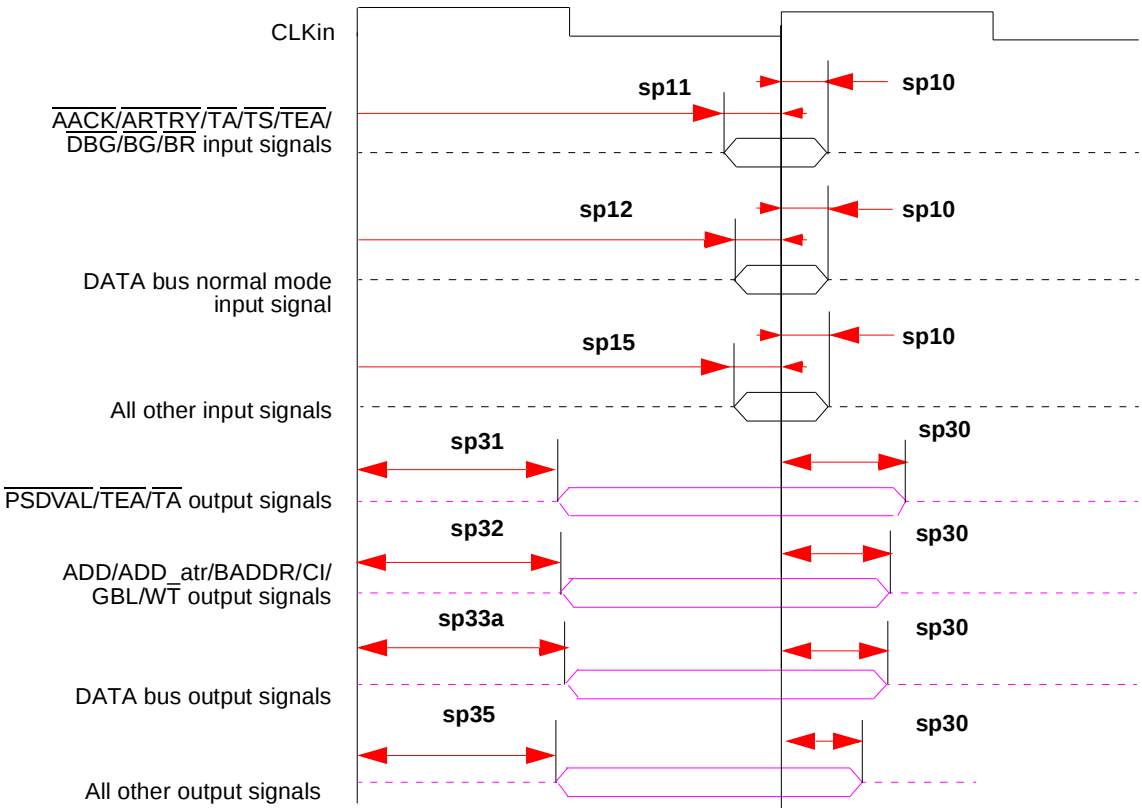
Figure 9. Bus Signals
