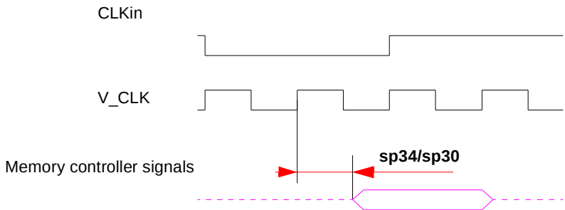
Figure 11. MEMC Mode Diagram
