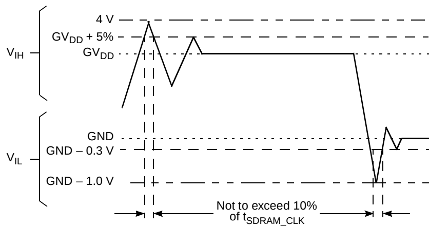
Figure 2. Overshoot/Undershoot Voltage
