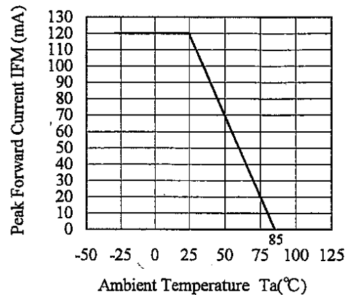
Peak Forward Current Derating Curve
